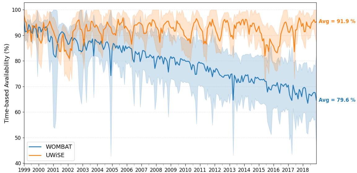
Figure 7. Comparison of average monthly time-based availability between WOMBAT and UWise. The shaded area represents \pm 1 standard deviation across 20 stochastic results.
