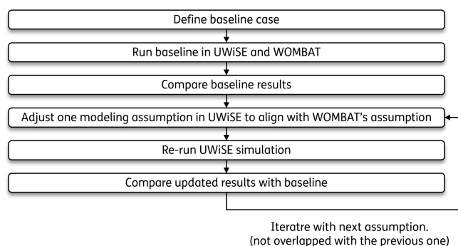
Figure 1. Overview of the verification process applied to O&M simulation models.
