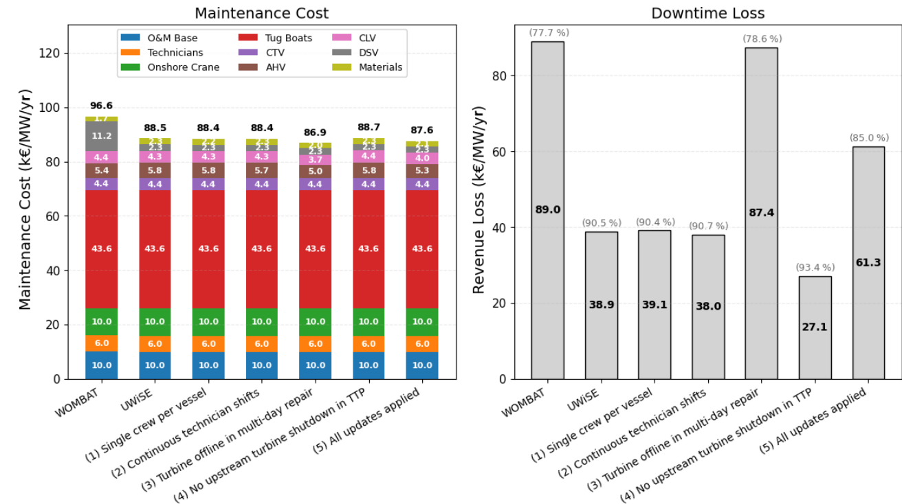
Figure 10. Comparison of maintenance cost, downtime loss, and energy-based availability between WOMBAT and UWise scenarios (baseline + 5 scenarios).
