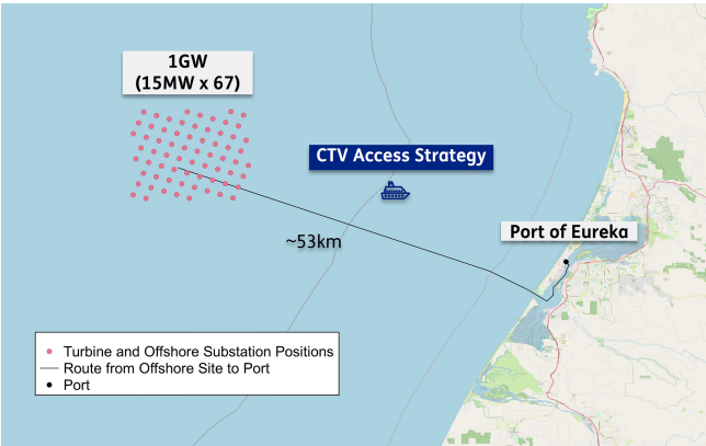
Figure 2. The wind farm layout of reference deep-water floating-wind-farm case. Background map: © OpenStreetMap contributors 2026 ( https://www.openstreetmap.org/copyright , last access: 11 February 2026).
