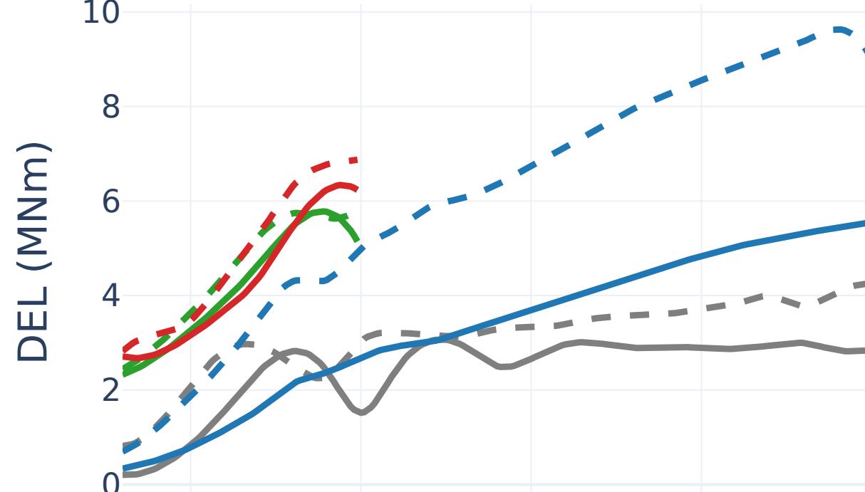
Main shaft bending x (MSBMX)
