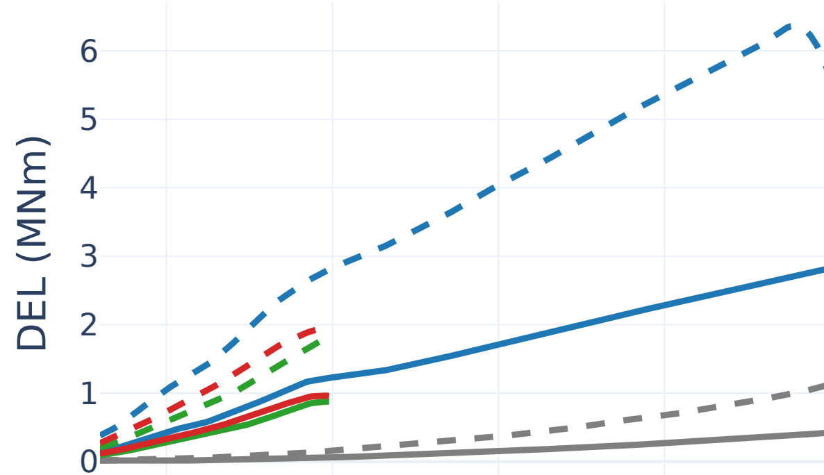
Blade root flapwise (BRFW)
