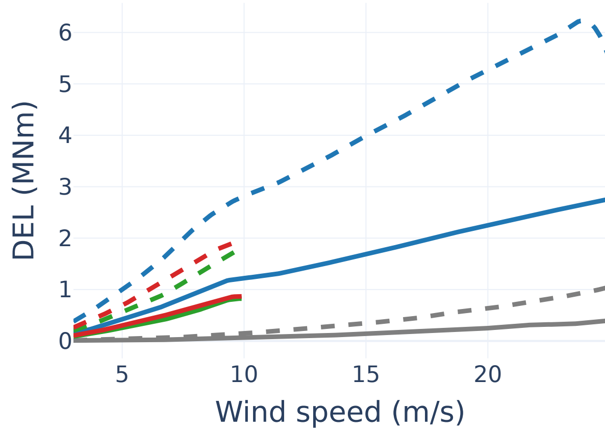
Main shaft bending x (MSBMX)
