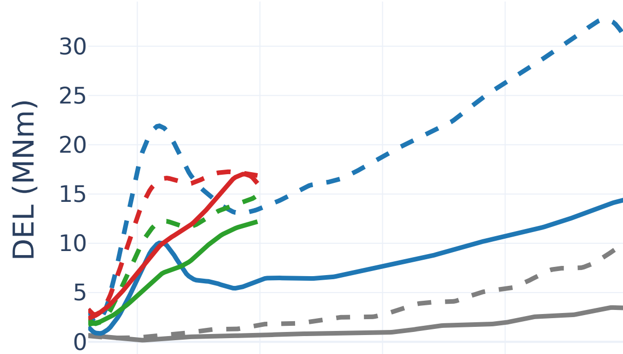
Tower top fore-aft (TTFA)
