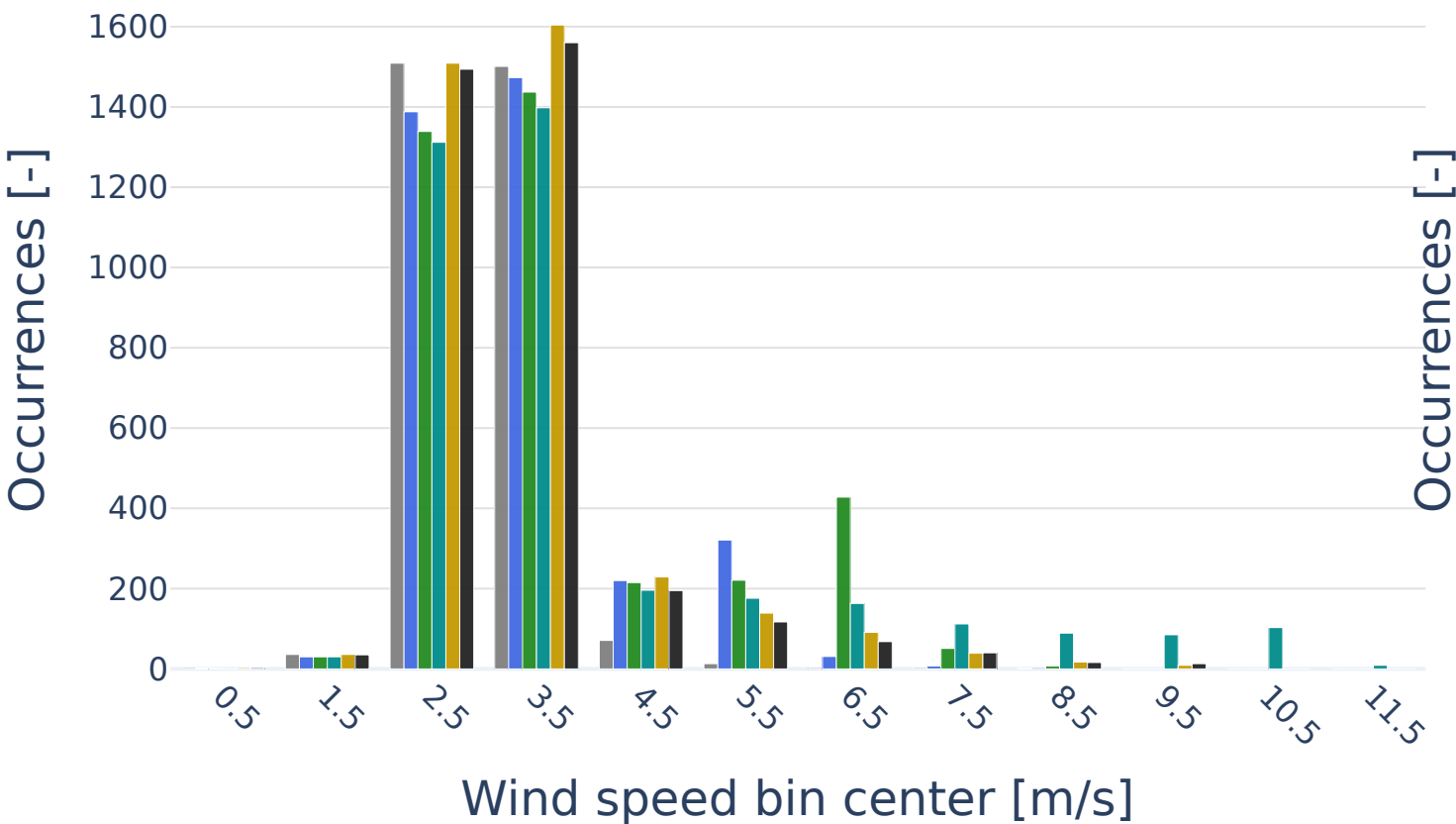
Wind speed distribution during startup/shutdown events
