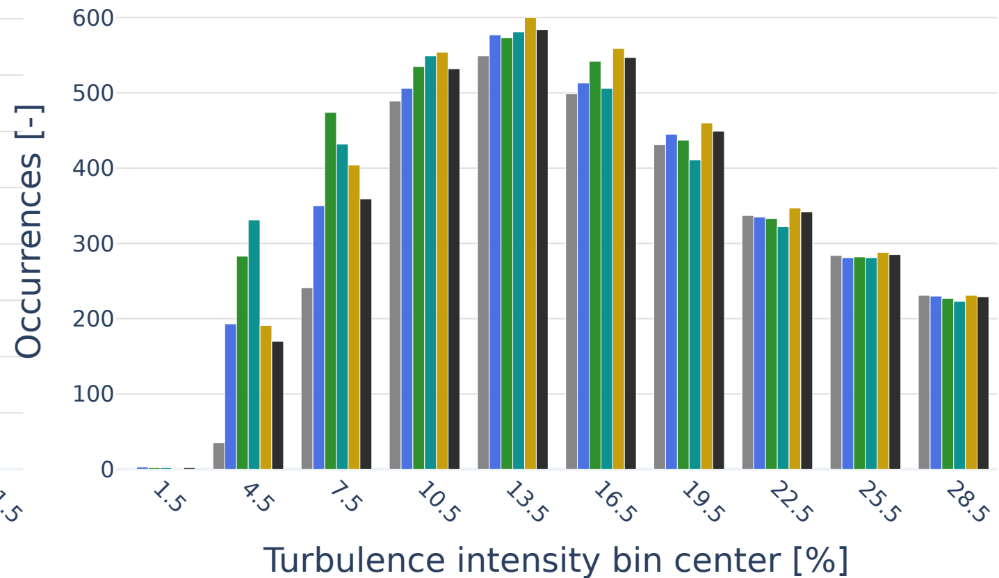
Turbulence intensity distribution during startup/shutdown events
