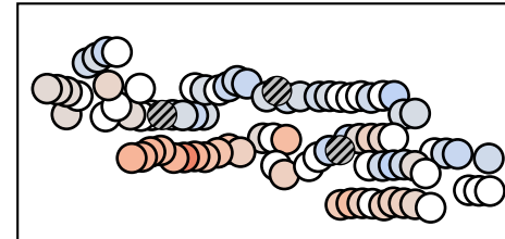
ID 8: Equinor WRF+EWP ensemble (mesoscale)
