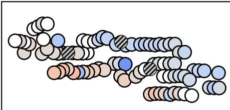
ID 7: Meteodyn WT TM 24h (RANS+Park1)
