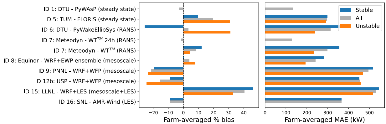
Figure S9. Histograms showing the farm-averaged percent bias (left) and mean absolute error (right) in modeled vs observed power produced by the King Plains wind plant on 24 August 2023 for each model submission to Phase 3 of the benchmark.
