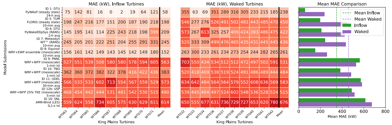
Figure S6. MAE in modeled power for selected turbines in the southern (inflow) row of King Plains (left) and the northern (waked) row (middle). The bar chart on the right compares the mean MAE across all submissions for inflow versus waked turbines. Results for phase 2.
