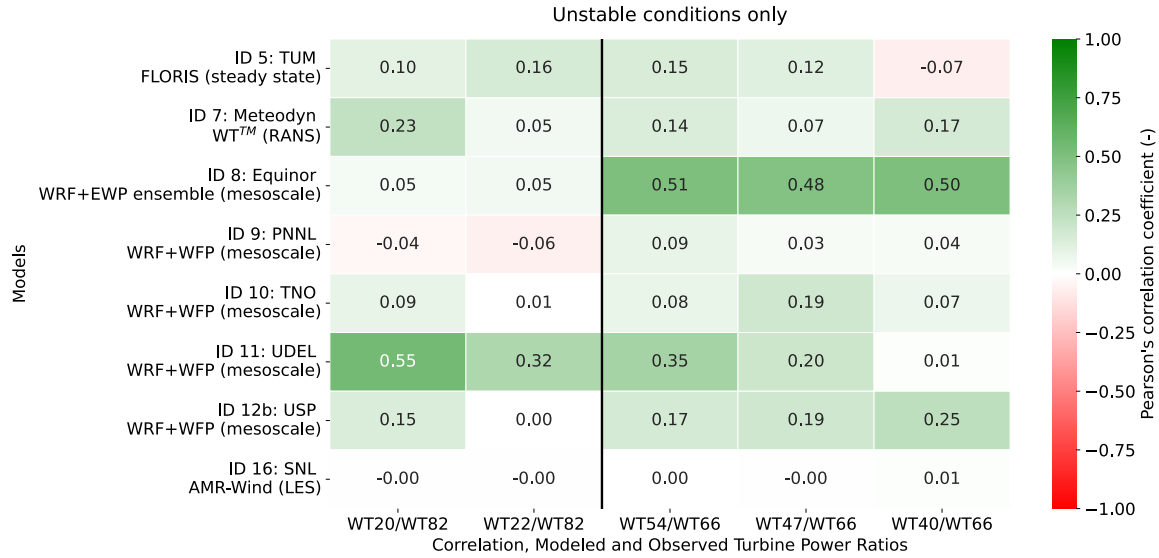
Figure S12. Pearson correlation coefficients between observed and modeled power ratios between turbine pairs during Phase 2, calculated using only data from unstable atmospheric conditions, for turbines in the western (left) and eastern (right) portions of King Plains.
