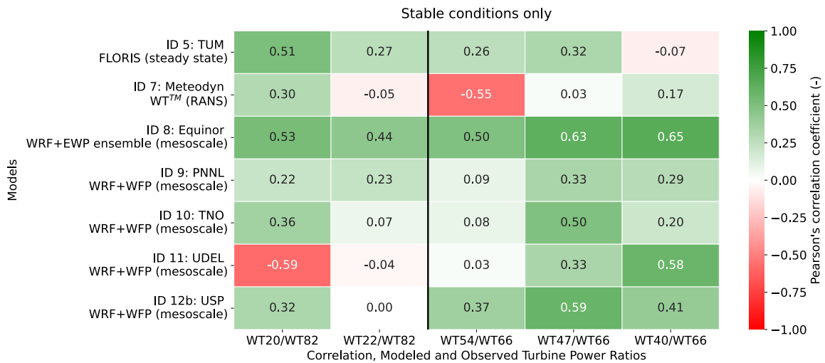
Figure S11. Pearson correlation coefficients between observed and modeled power ratios between turbine pairs during Phase 2, calculated using only data from stable atmospheric conditions, for turbines in the western (left) and eastern (right) portions of King Plains.
