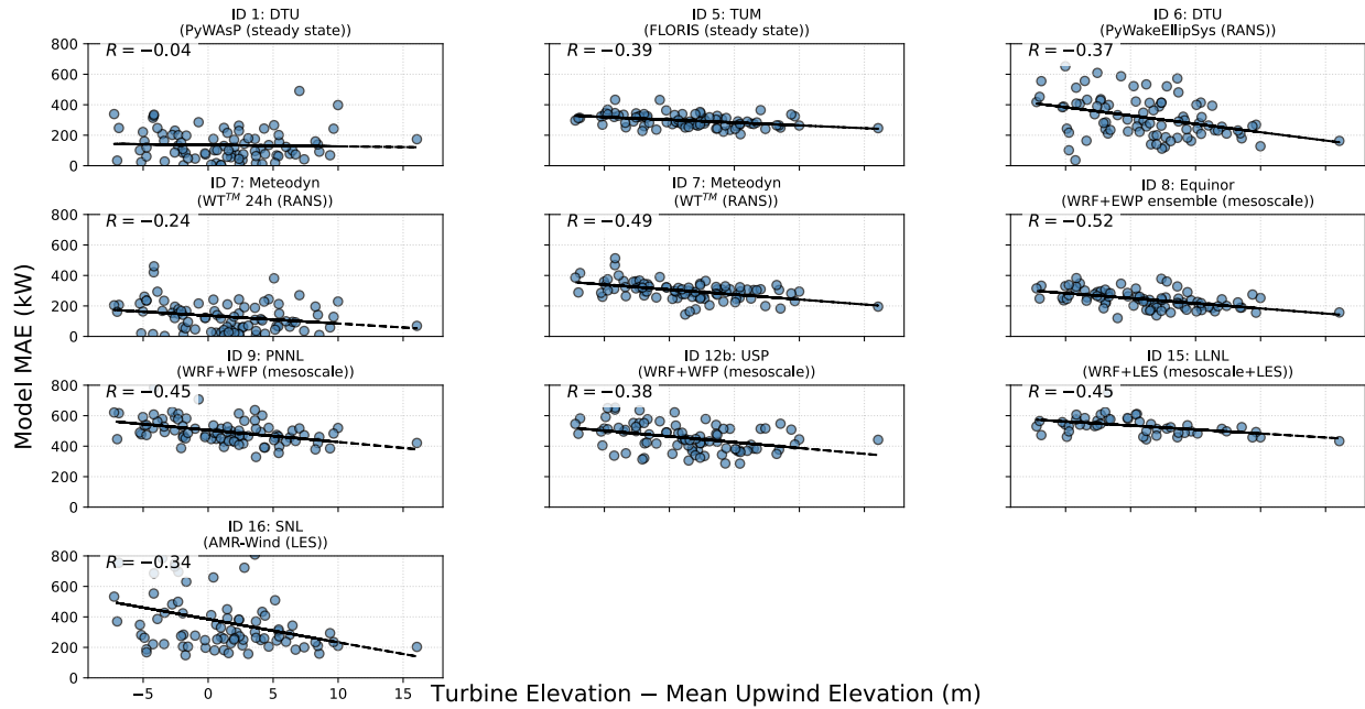
Figure S4. Scatterplots of turbine-level Mean Absolute Error (MAE) versus relative terrain elevation for each Phase 3 model submission.
