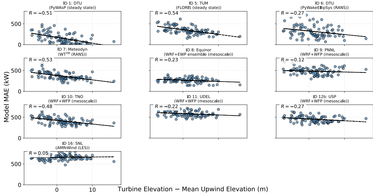
Figure S3. Scatterplots of turbine-level Mean Absolute Error (MAE) versus relative terrain elevation for each Phase 2 model submission.
