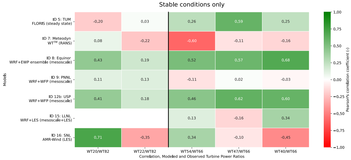
Figure S14. Pearson correlation coefficients between observed and modeled power ratios between turbine pairs during Phase 3, calculated using only data from stable atmospheric conditions, for turbines in the western (left) and eastern (right) portions of King Plains.
