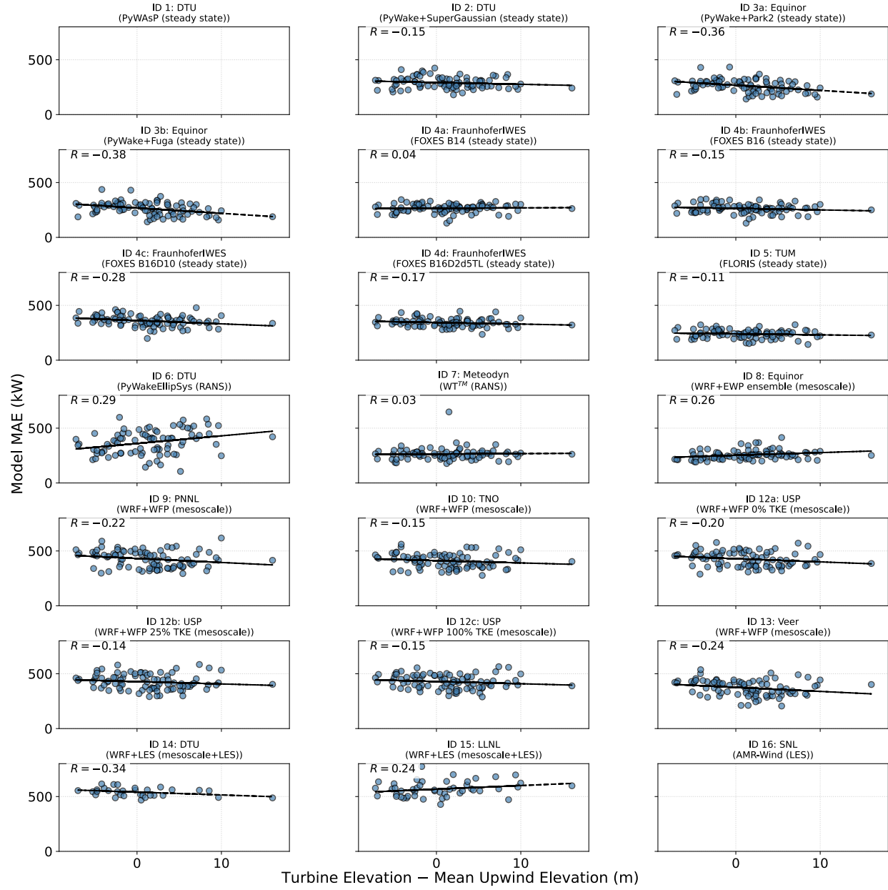
Figure S2. Scatterplots of turbine-level Mean Absolute Error (MAE) versus relative terrain elevation for each Phase 1 model submission (unstable conditions only).
