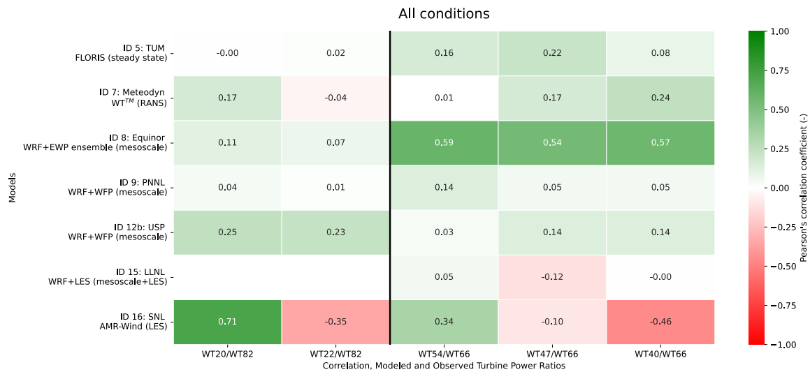
Figure S13. Pearson correlation coefficients between observed and modeled power ratios for selected turbine pairs during Phase 3. The ratios are calculated as the power of the waked turbine divided by the power of a corresponding upstream reference turbine in the southernmost row, for turbines in the western (left) and eastern (right) portions of King Plains.
