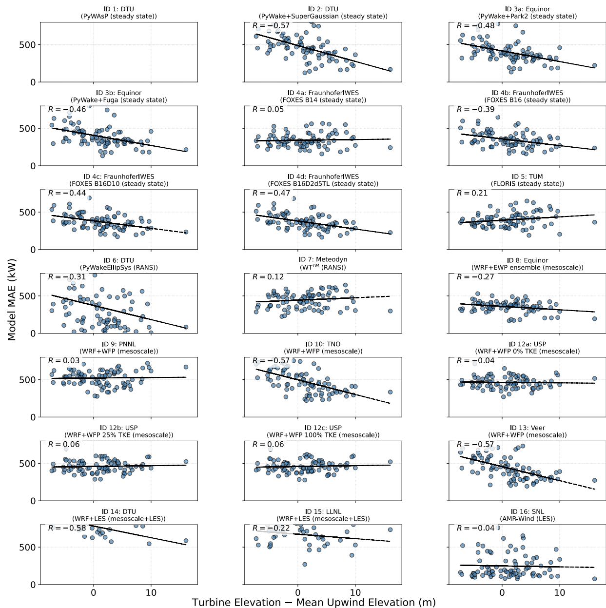
Figure S1. Scatterplots of turbine-level Mean Absolute Error (MAE) versus relative terrain elevation for each Phase 1 model submission (stable conditions only).
