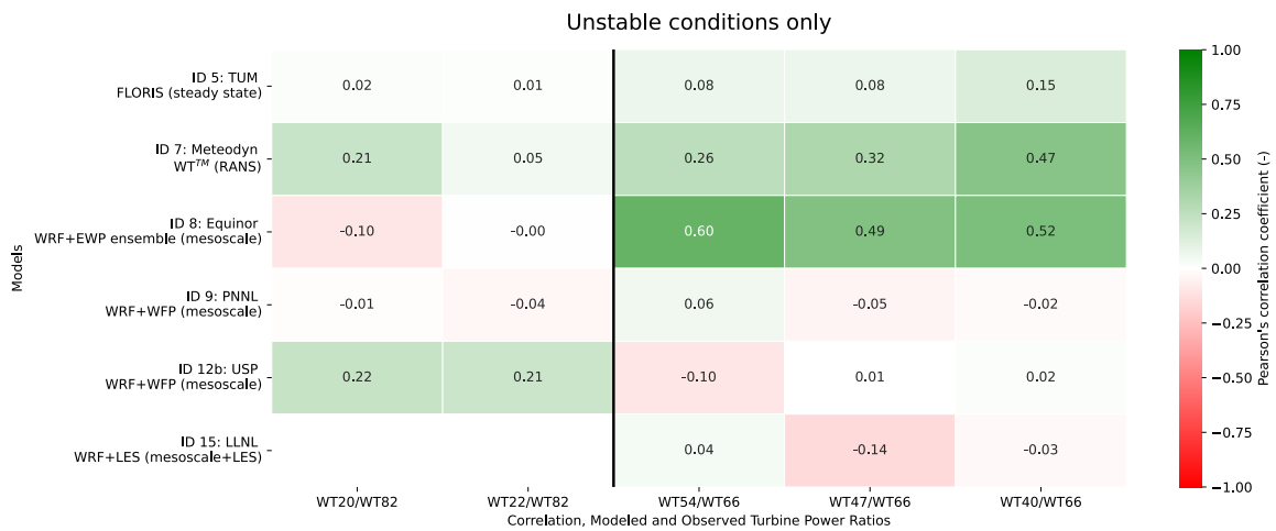
Figure S15. Pearson correlation coefficients between observed and modeled power ratios between turbine pairs during Phase 3, calculated using only data from unstable atmospheric conditions, for turbines in the western (left) and eastern (right) portions of King Plains.
