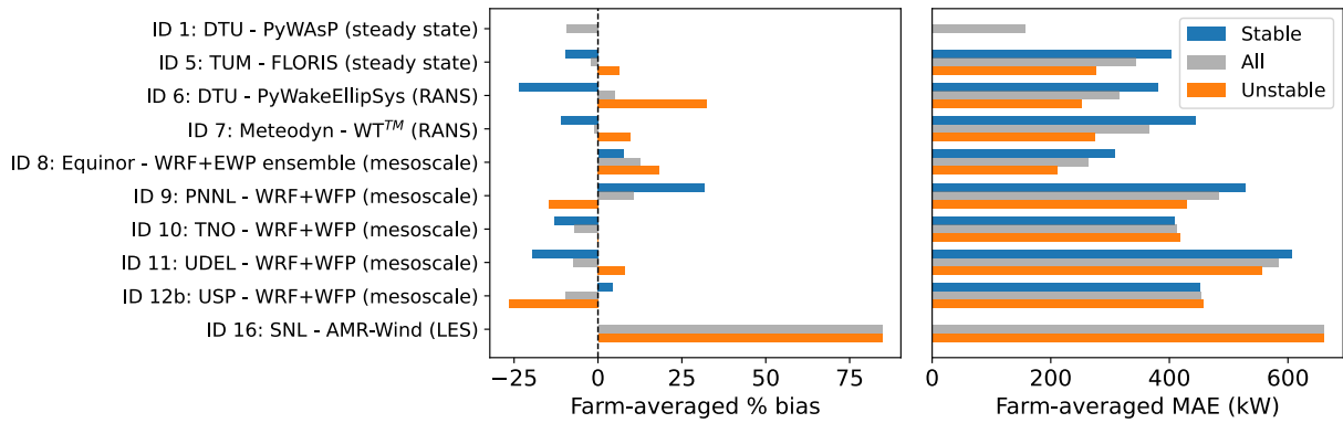
Figure S8. Histograms showing the farm-averaged percent bias (left) and mean absolute error (right) in modeled vs observed power produced by the King Plains wind plant on 24 August 2023 for each model submission to Phase 2 of the benchmark.
