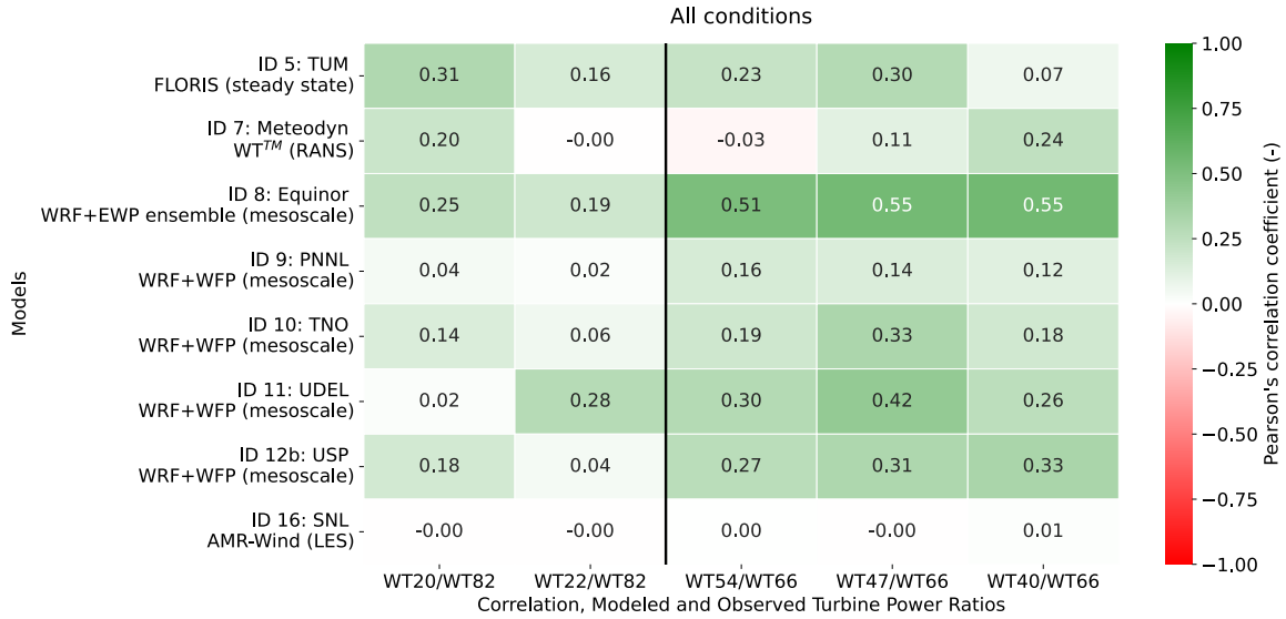
Figure S10. Pearson correlation coefficients between observed and modeled power ratios for selected turbine pairs during Phase 2. The ratios are calculated as the power of the waked turbine divided by the power of a corresponding upstream reference turbine in the southernmost row, for turbines in the western (left) and eastern (right) portions of King Plains.
