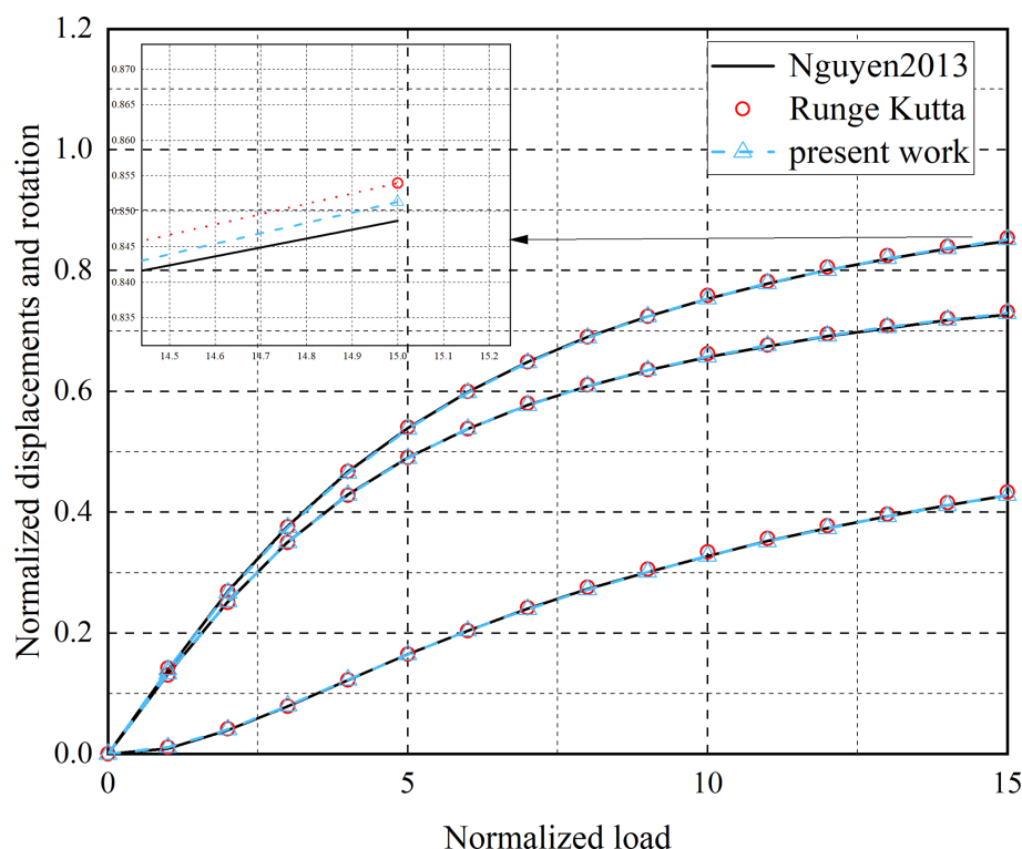
Figure 8. Normalized moment and deformation in tapered beam.
