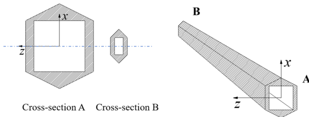
Figure 10. Column geometry.
