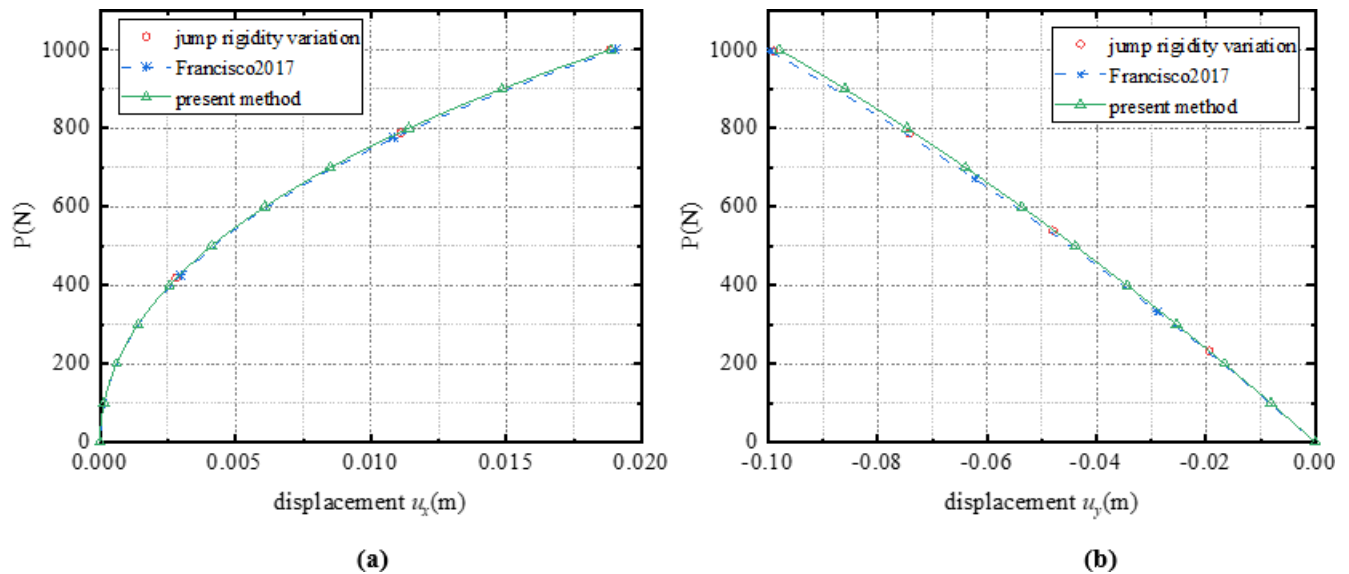
Figure 11. Frame displacement at node 13: (a) u_x displacement at node 13, (b) u_y displacement at node 13.
