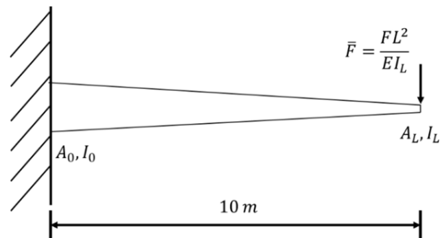
Figure 7. Conical beam.
