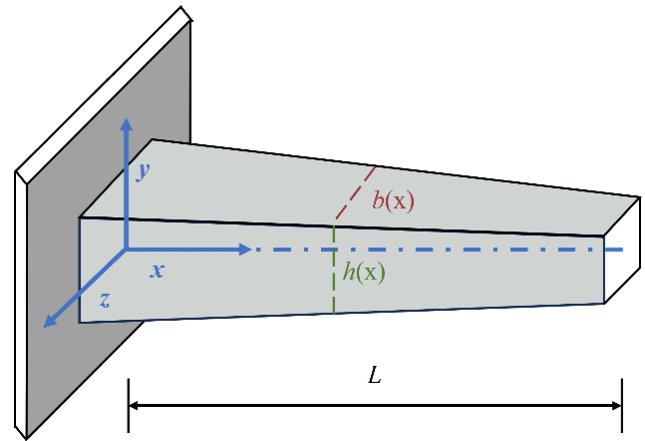
Figure 1. Variable geometric properties in a tapered beam.
