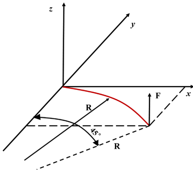
Figure 4. Pre-bent cantilever beam.
