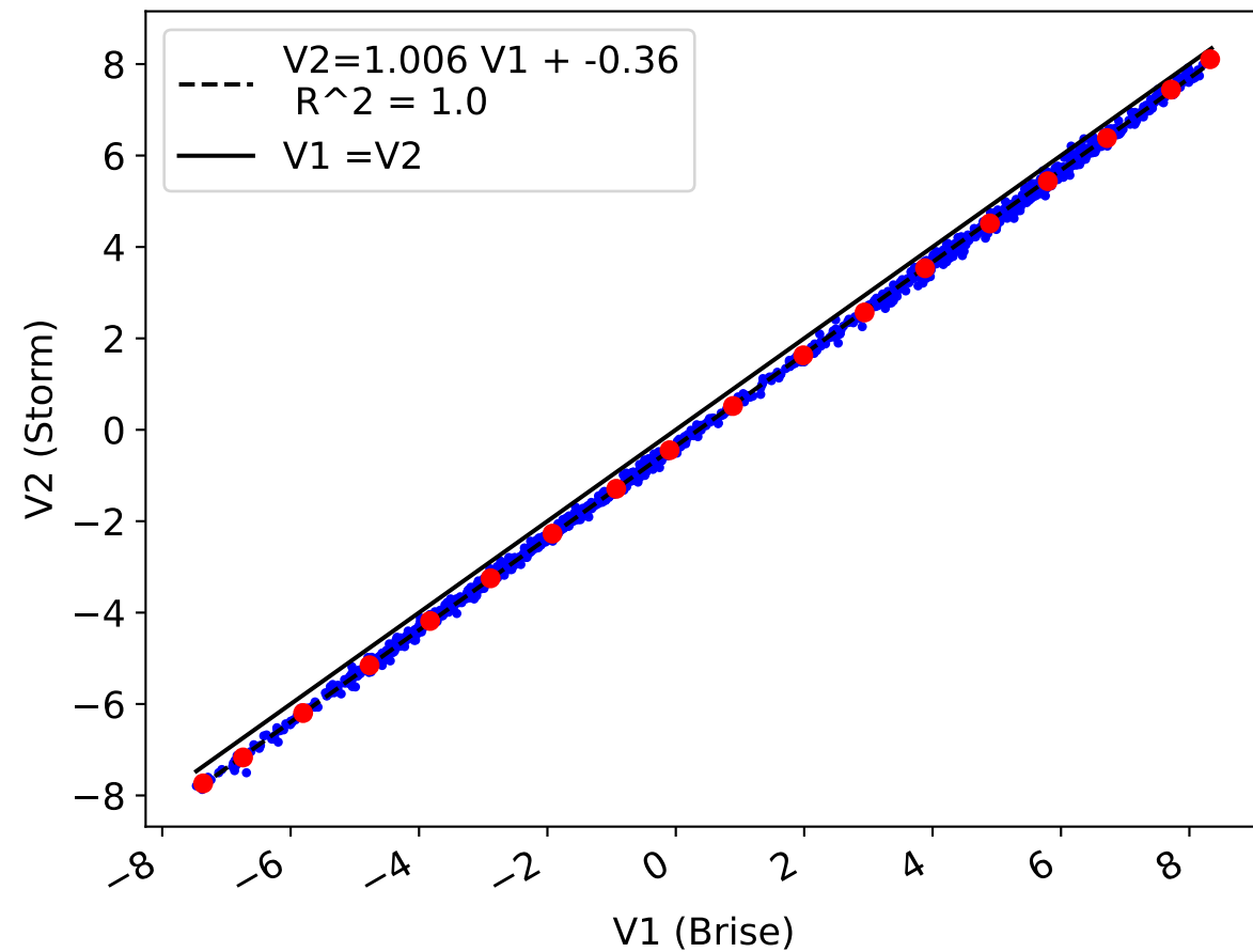
Brise vs Storm at 700.5 m No. of points: 1687
