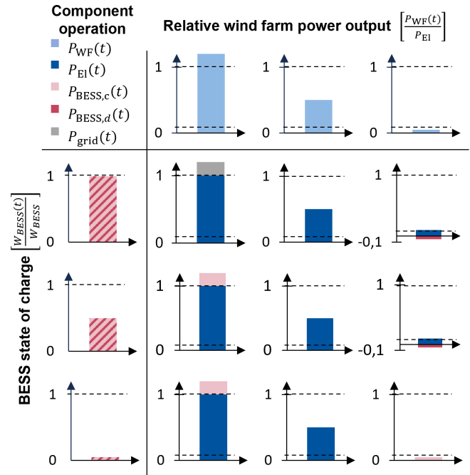
Figure 2. Power flows of HPP components for the determined operation strategy for a time step depending on the relative WF power output (top row) and the BESS state of charge (left column).
