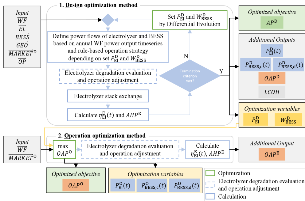
Figure 1. Schematic overview of the proposed design methodology (superscript index D) and the subsequent MIL operation optimization (superscript index O) with post-optimization degradation evaluation (superscript index E).
