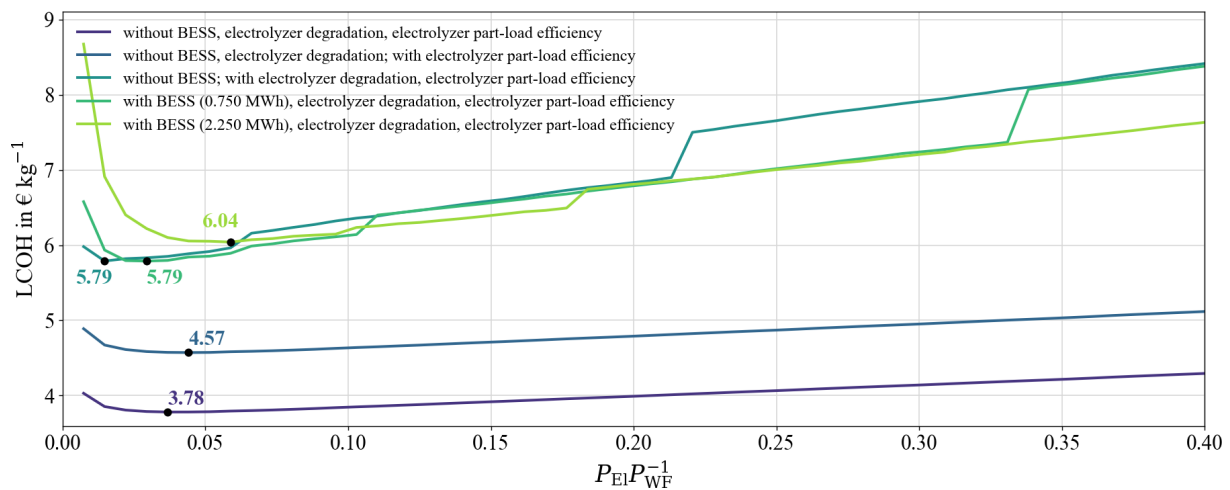
Figure 8. LCOH over the ratio of electrolyzer rated power to wind farm rated power for four different modeling approaches and two different BESS sizes.
