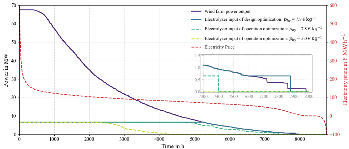
Figure 10. Sorted load duration curves of the WF power output, the electrolyzer power input of the design optimization and for the MIL operation optimization for two different hydrogen price scenarios, and the sorted electricity price over 1 year.
