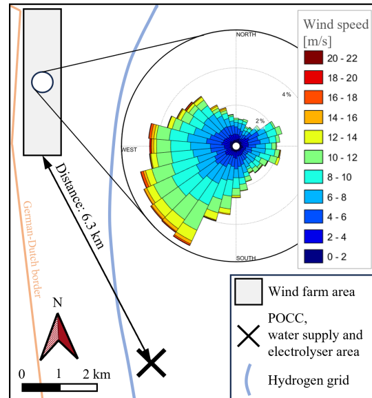
Figure 5. Schematic illustration of the wind farm site and its distance to the POCC, the water supply, and the location of the electrolyzer. Also shown is a part of the planned German hydrogen grid and the wind rose at the center of the wind farm site at 100 m height above ground level.
