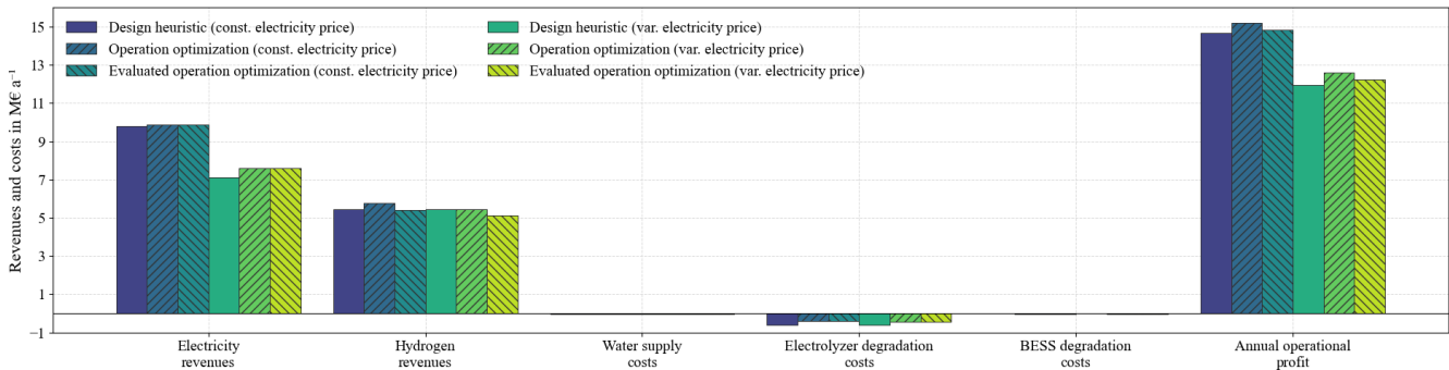
Figure 9. Comparison of the annual operational profit and its proportions in the design optimization, the MIL operation optimization, and its degradation evaluation for constant and variable electricity prices.
