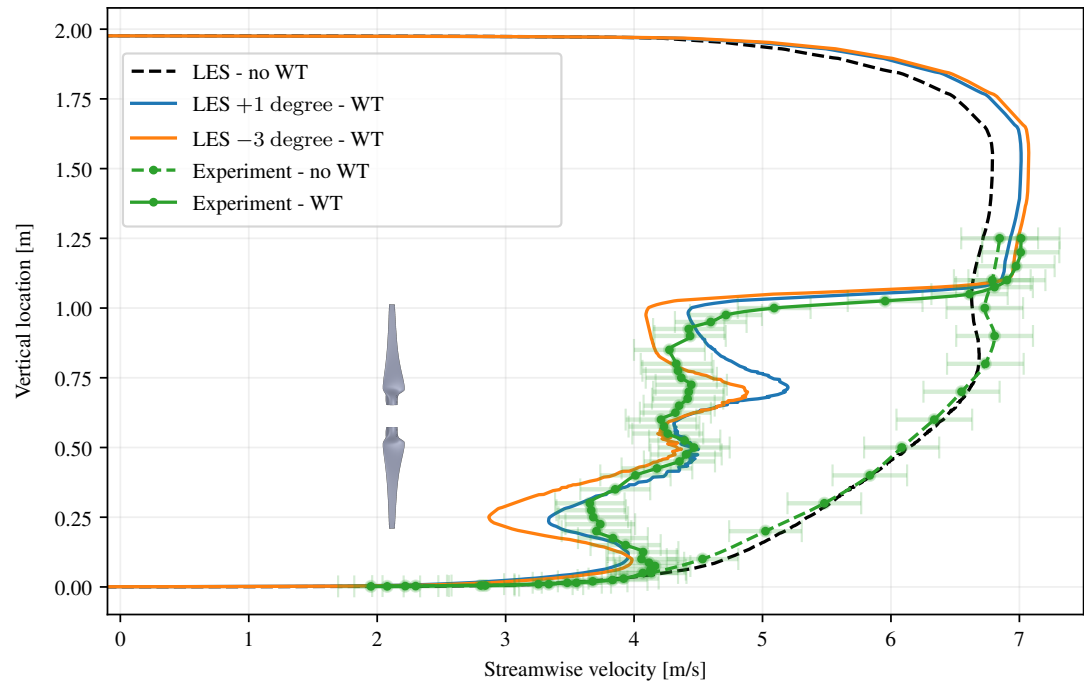
Velocity at location 2 ( 1.41 D downstream)
