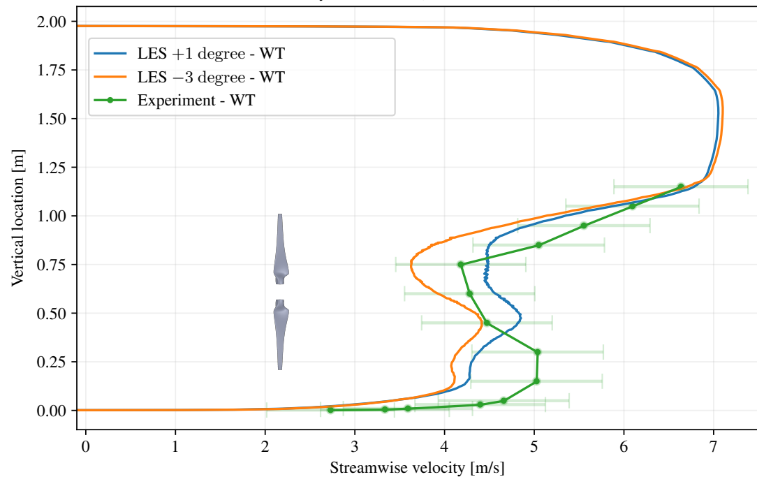
Velocity at location 3 ( 4.35 D downstream)
