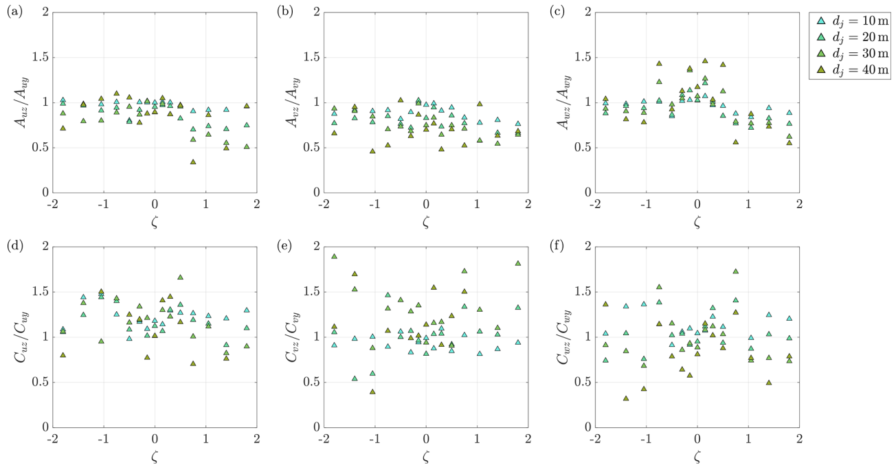
Figure 23. Ratio of vertical to lateral (a–c) scaling coefficients and (d–f) decay coefficients for separations of d_j = 10 to 40 m and mean heights of \bar{z} = 120 to 130 m.
