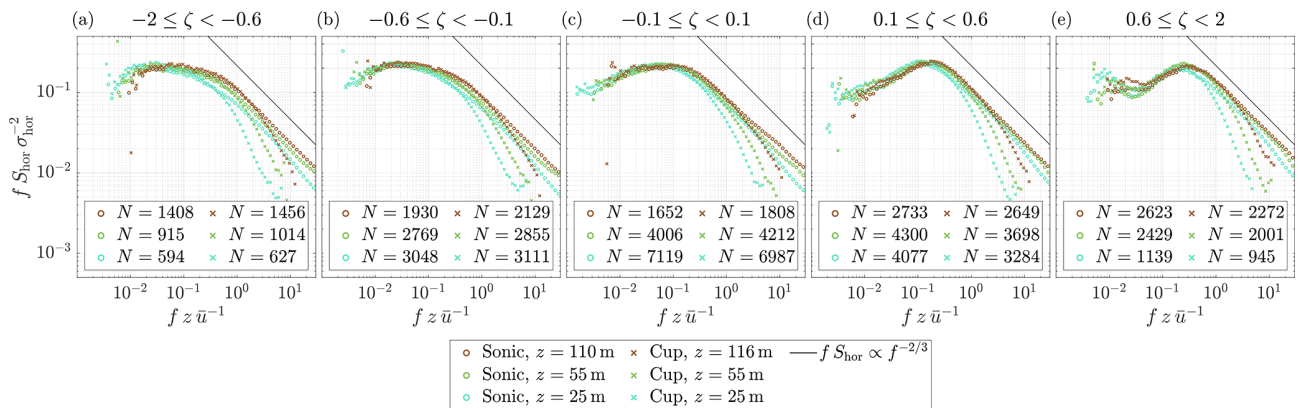
Figure 13. Ensemble-averaged horizontal wind speed spectra from sonic and cup anemometers under (a) highly unstable to (e) highly stable conditions.
