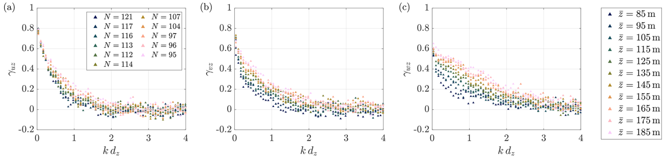
Figure 19. Vertical co-coherence of (a) along-wind, (b) cross-wind, and (c) vertical velocity from SRWS as a function of the average measurement height \bar{z} for a vertical separation of d_z = 60 m under neutral conditions.
