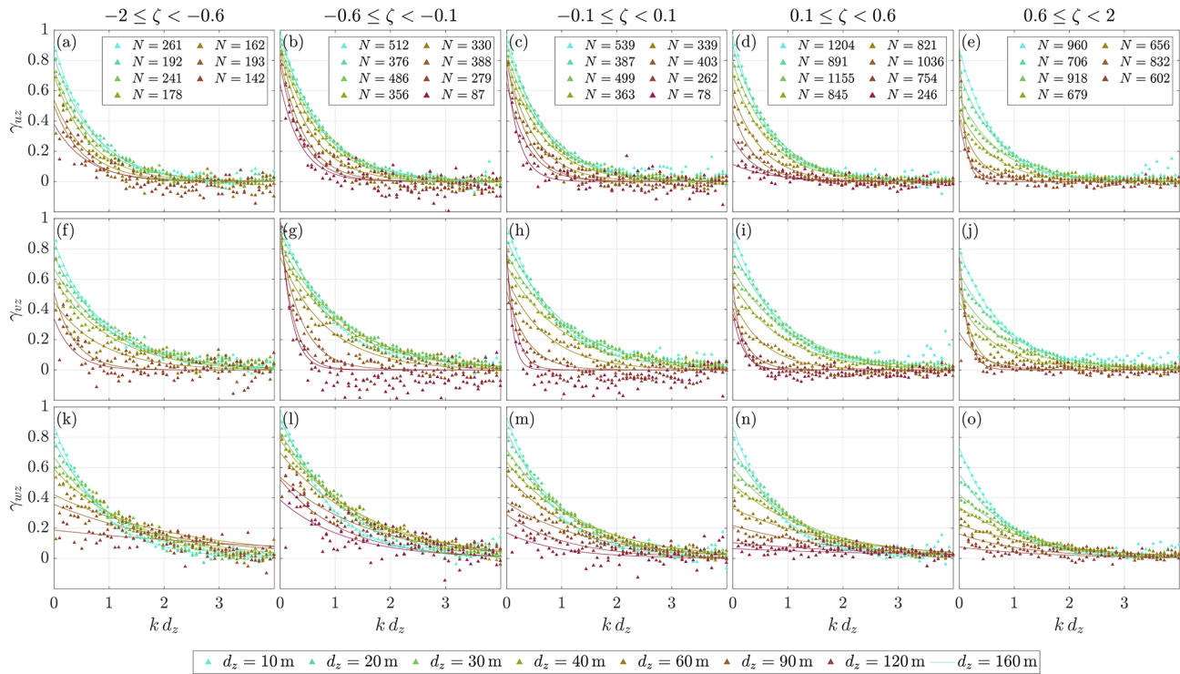
Figure 18. Vertical co-coherence of (a–e) along-wind, (f–j) cross-wind, and (k–o) vertical velocity from SRWS for separations ranging from 10 to 160 m under highly unstable (left) to highly stable (right) conditions and average heights of 110 \text{ m} \leq \bar{z} \leq 140 \text{ m} . The 160 m separation is omitted for |\zeta| > 0.6 due to high uncertainty associated with a limited sample size.
