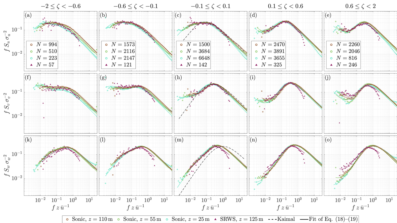
Figure 14. Ensemble-averaged (a–e) along-wind, (f–j) cross-wind, and (k–o) vertical velocity spectra from sonic anemometers and SRWS under highly unstable (left) to highly stable (right) conditions.
