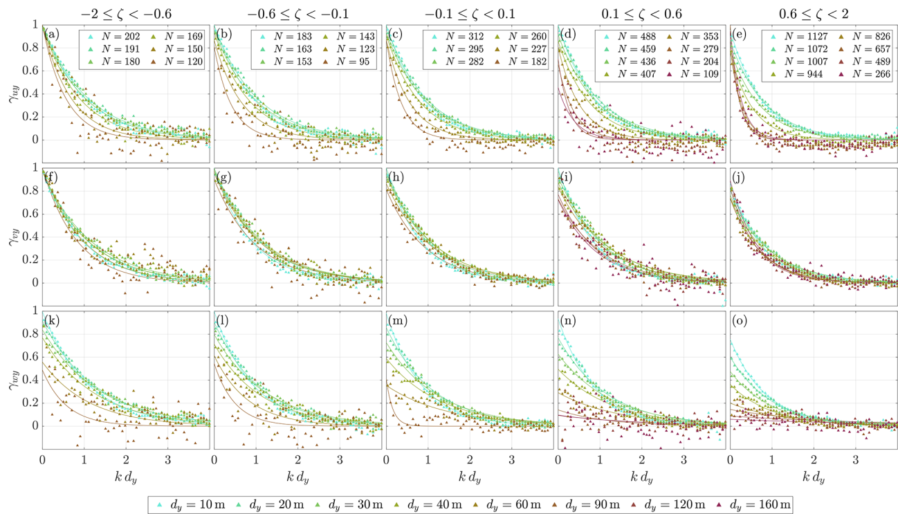
Figure 21. Lateral co-coherence of (a–e) along-wind, (f–j) cross-wind, and (k–o) vertical velocity from SRWS for separations ranging from 10 to 160 m under highly unstable (left) to highly stable (right) conditions and a measurement height of 125 m. The 120 and 160 m separations are omitted for \zeta < 0.1 due to high uncertainty associated with a limited sample size.
