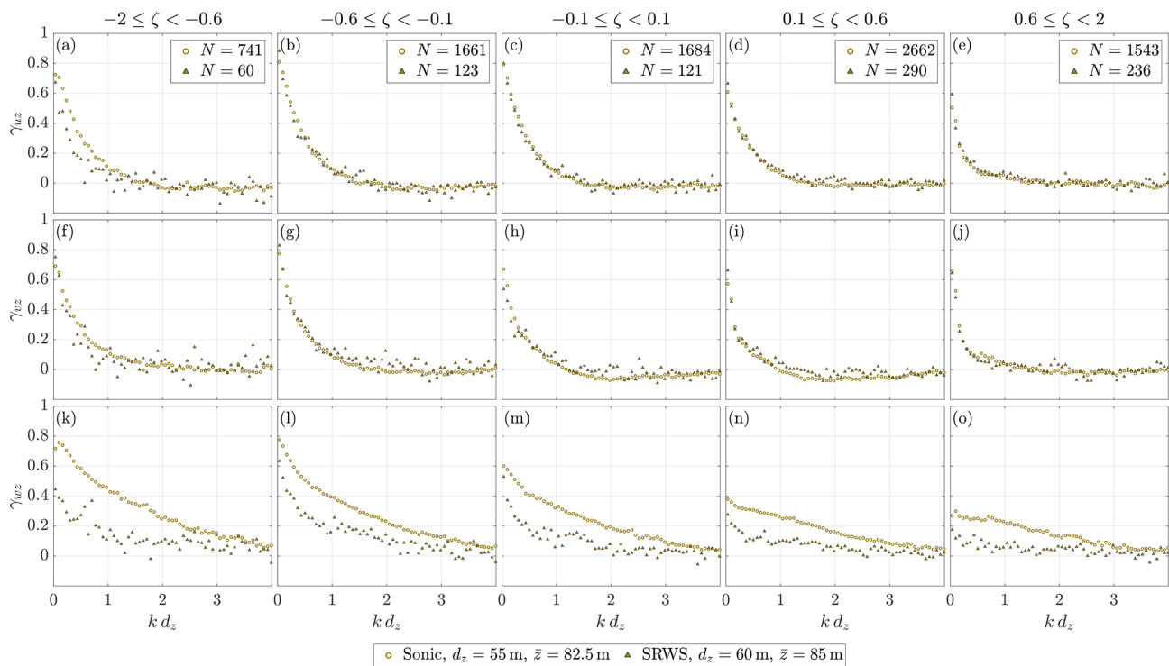
Figure 17. Vertical co-coherence of (a–e) along-wind, (f–j) cross-wind, and (k–o) vertical velocity from sonic anemometers and SRWS at comparable separations and measurement heights under highly unstable (left) to highly stable (right) conditions.
