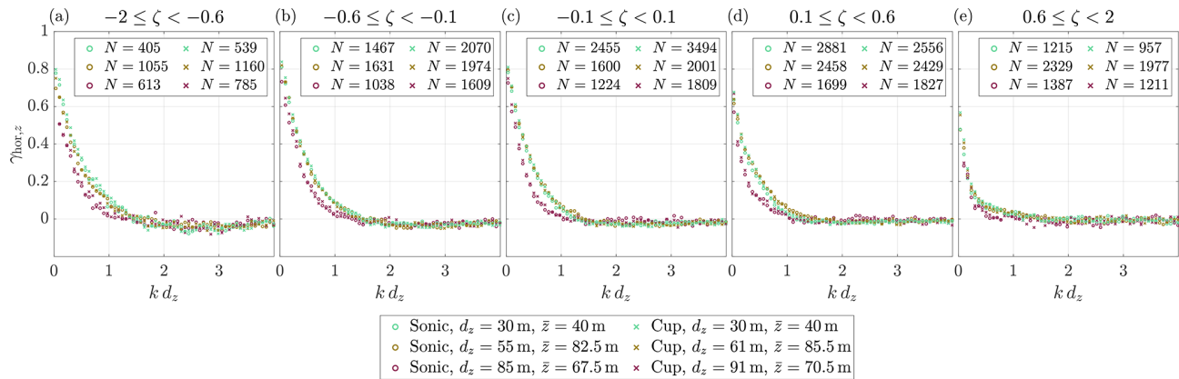
Figure 16. Vertical co-coherence of horizontal wind speed from sonic and cup anemometers under (a) highly unstable to (e) highly stable conditions.
