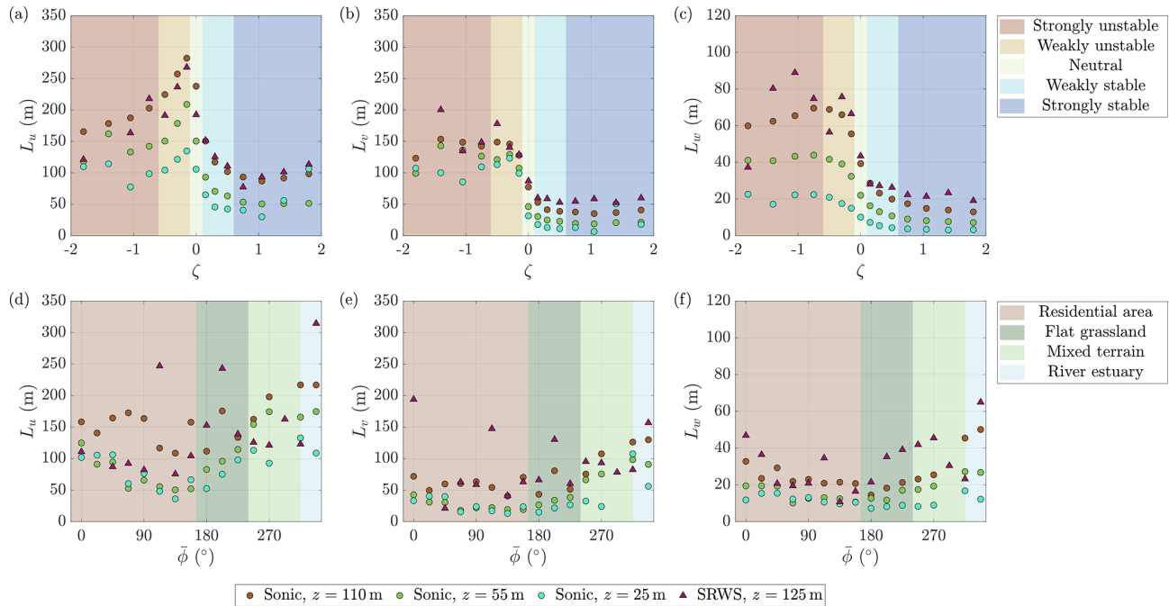
Figure 10. Median integral length scales derived from the auto-correlation function as a function of (a–c) atmospheric stability and (d–f) wind direction. Panels (c) and (f) use a reduced y-axis scale for the vertical length scale L_w for improved readability.
