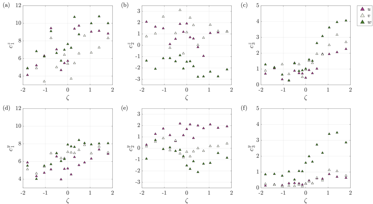
Figure B1. Empirical model coefficients for computation of (a–c) vertical and (d–f) lateral coherence of the along-wind, cross-wind, and vertical velocity components. Values are obtained from least-square fits of Eq. (B1) to the SRWS measurements.
