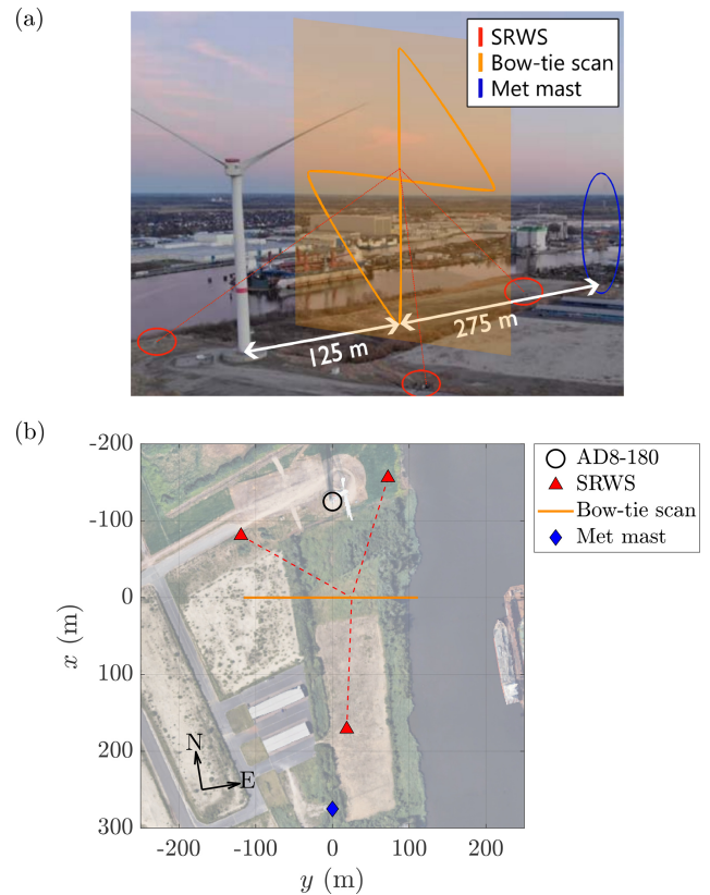
Figure 3. (a) Aerial view of the test site and (b) plan view showing the sensor locations in a fixed reference frame. Background imagery © Google, map data © 2009 GeoBasis-DE/BKG. Markers added by the authors.
