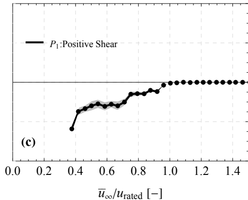
REWS (wind lidar)
