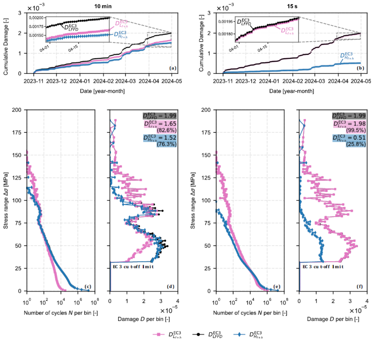
Figure 12. FA-direction fatigue at tower section T1 (6 months, 6.25 Hz): residual-preserving LFFD versus conventional window-based counting. (a–b) Cumulative damage for 10 min and 15 s windows. (c, e) \Delta\sigma - N spectra and (d, f) \Delta\sigma - D spectra at the end of the 6 months, for 10 min and 15 s windows respectively. Curves compare LFFD total damage (baseline), the LFFD low-frequency contribution, and conventional window-based high-cycle counting. Percentages indicate damage relative to the LFFD baseline (Eq. 5, EC3). Insets show a close-up view of the final month of the monitoring period (15 s panel restricted to LFFD total and low-frequency, for clarity). Damage is computed using EC3 detail category 80, employing a bi-linear formulation with slopes m = 3/5 .
