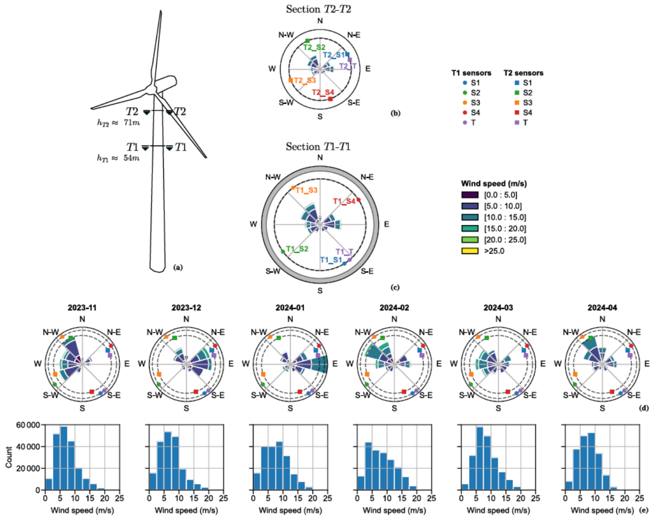
Figure 4. Turbine instrumentation and inflow conditions. (a) Instrumented tower sections T1 and T2. (b–c) Sensor layout at each section (strain gauges S1–S4 and temperature sensor T ). (d) Monthly wind roses and (e) wind speed histograms for November 2023–April 2024.
