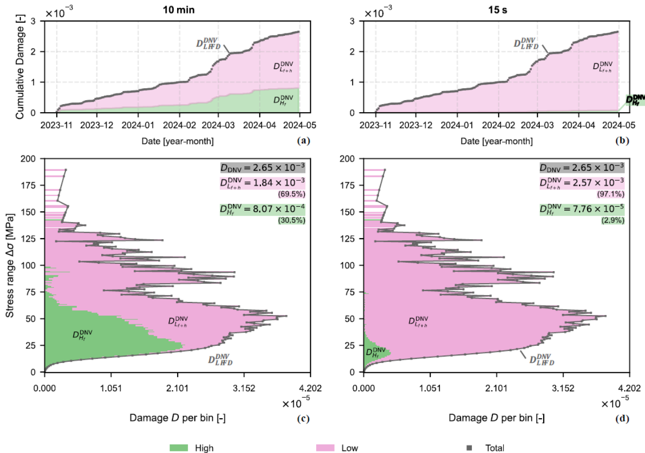
Figure 11. FA-direction fatigue at tower section T1 (6 months, 50 Hz), computed using the DNV welded-steel \sigma - N curve (bi-linear formulation, slopes m = 3/5 ). (a–b) Cumulative damage for 10 min and 15 s windows. (c–d) Final \Delta\sigma - D spectra. Total damage is decomposed into within-window full-cycle damage (green) and residual-based damage (pink). The percentages of damage are computed by Eq. (2).
