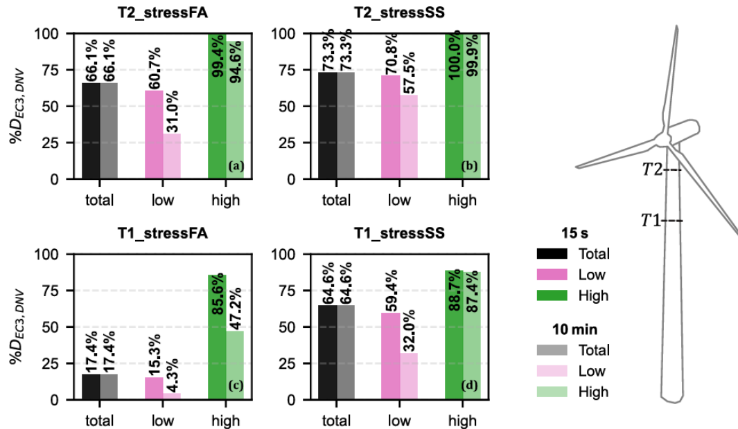
Figure 7. Relative differences between fatigue-damage estimates obtained using Eurocode 3 (EC3) and DNVGL-RP-C203 (DNV) for 10 min and 15 s windows. Damage is computed using EC3 detail category 80 and DNVGL-RP-C203 welded-steel \sigma - N curves, both employing a bi-linear formulation with slopes m = 3/5 . Results are shown for tower section T1 (near-base) and T2 (upper tower) in the fore-aft (FA) and side-to-side (SS) directions: (a) T2-FA, (b) T2-SS, (c) T1-FA, (d) T1-SS. Bars indicate percentage differences in accumulated damage between EC3 and DNV for the total fatigue damage and for the low- and high-frequency contributions, computed using Eq. (3).
