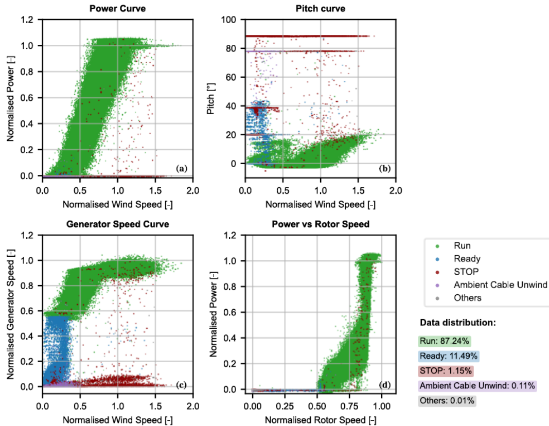
Figure 5. SCADA operational curves for the study period (15 s data). (a–c) Normalised power, pitch, and generator-speed curves versus normalised wind speed. (d) Normalised power versus normalised rotor speed. Colours indicate operational status; the right panel shows the sample distribution by status.
