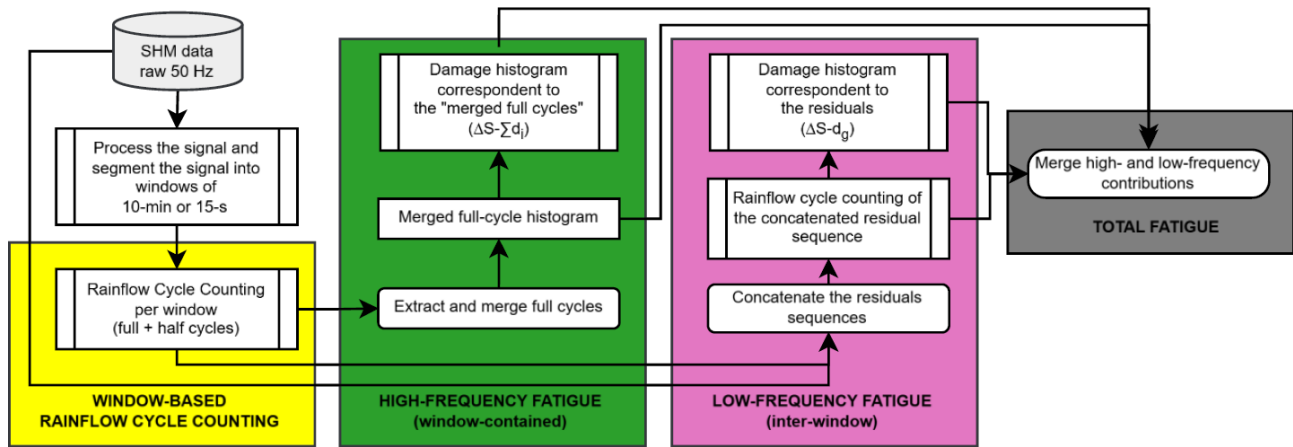
Figure 2. Simplified flowchart of the modified low-frequency fatigue dynamics (LFFD) methodology, inspired in Faria et al. (2024), Sadeghi et al. (2022). Following signal pre-processing and windowing, rainflow cycle counting (RFC) is applied independently within each window. High-frequency fatigue (green) is obtained from merged full-cycle histograms, while low-frequency fatigue (pink) is derived from RFC applied to concatenated residual sequences across windows. Damage and cycle-count histograms are computed separately for each contribution and subsequently merged to obtain the total fatigue response (grey), preserving equivalence with continuous rainflow counting. The link from the raw SHM data to the residual-concatenation step reflects the need for the original, temporally ordered stress values of the unclosed excursions, which are not retained in the half-cycle counts alone.
