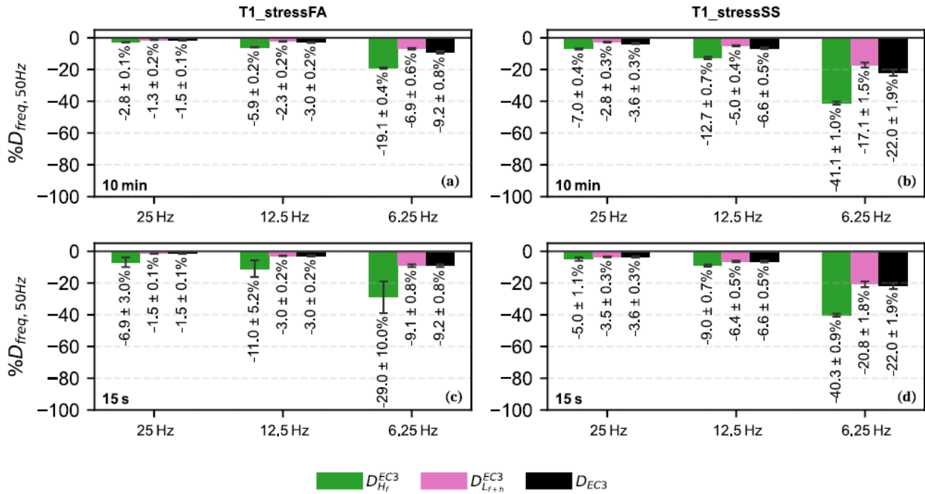
Figure 9. Relative damage loss with respect to 50 Hz at tower section T1 for fore–aft (FA) and side-to-side (SS), computed by Eq. (4). Bars show total, low-frequency, and high-frequency contributions for 25, 12.5, and 6.25 Hz, using 10 min and 15 s windows. Values are 6-month means with standard deviations. Damage computed with EC3 detail category 80 curve.
