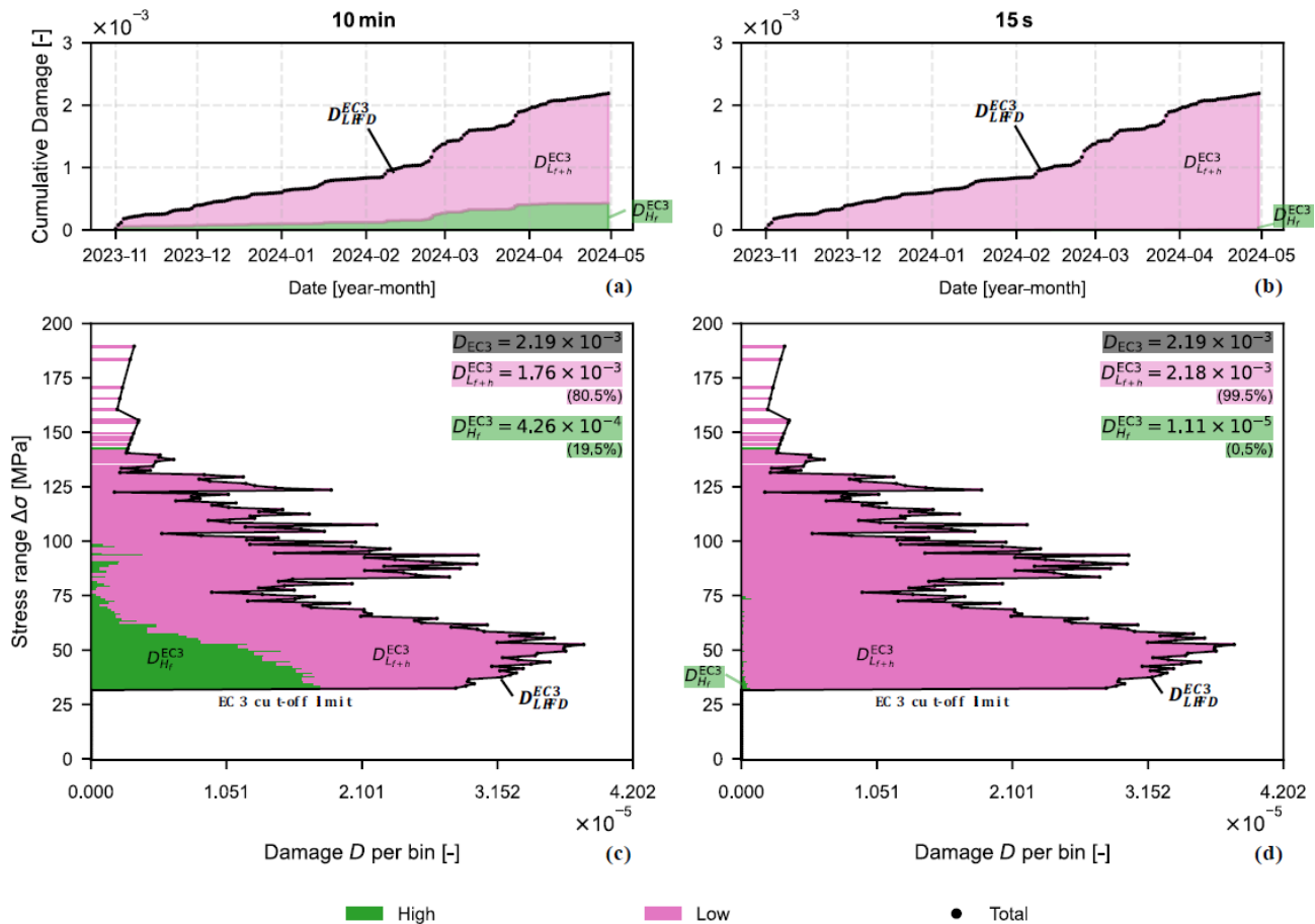
Figure 10. FA-direction fatigue at tower section T1 (6 months, 50 Hz), computed using the EC3 detail category 80 \sigma - N curve (bilinear formulation, slopes m = 3/5 ). (a–b) Cumulative damage for 10 min and 15 s windows. (c–d) Final \Delta\sigma - D spectra. Total damage is decomposed into within-window full-cycle damage (green) and residual-based damage (pink). The percentages of damage are computed by Eq. (2).
