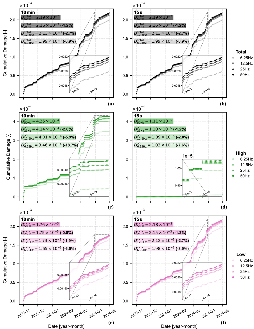
Figure 8. Cumulative FA-direction damage at tower section T1 for four sampling rates (50, 25, 12.5 and 6.25 Hz) and two window lengths, shown separately for each fatigue component: (a, b) total, (c, d) high-frequency, and (e, f) low-frequency contributions computed with EC3 detail category 80 curve. Columns (a), (c), (e) correspond to the 10 min and (b), (d), (f) to 15 s window lengths. Annotations report end-of-period values and deviations from the 50 Hz baseline, computed by Eq. (4). Insets show a close-up view of the final month of the analysis period.
