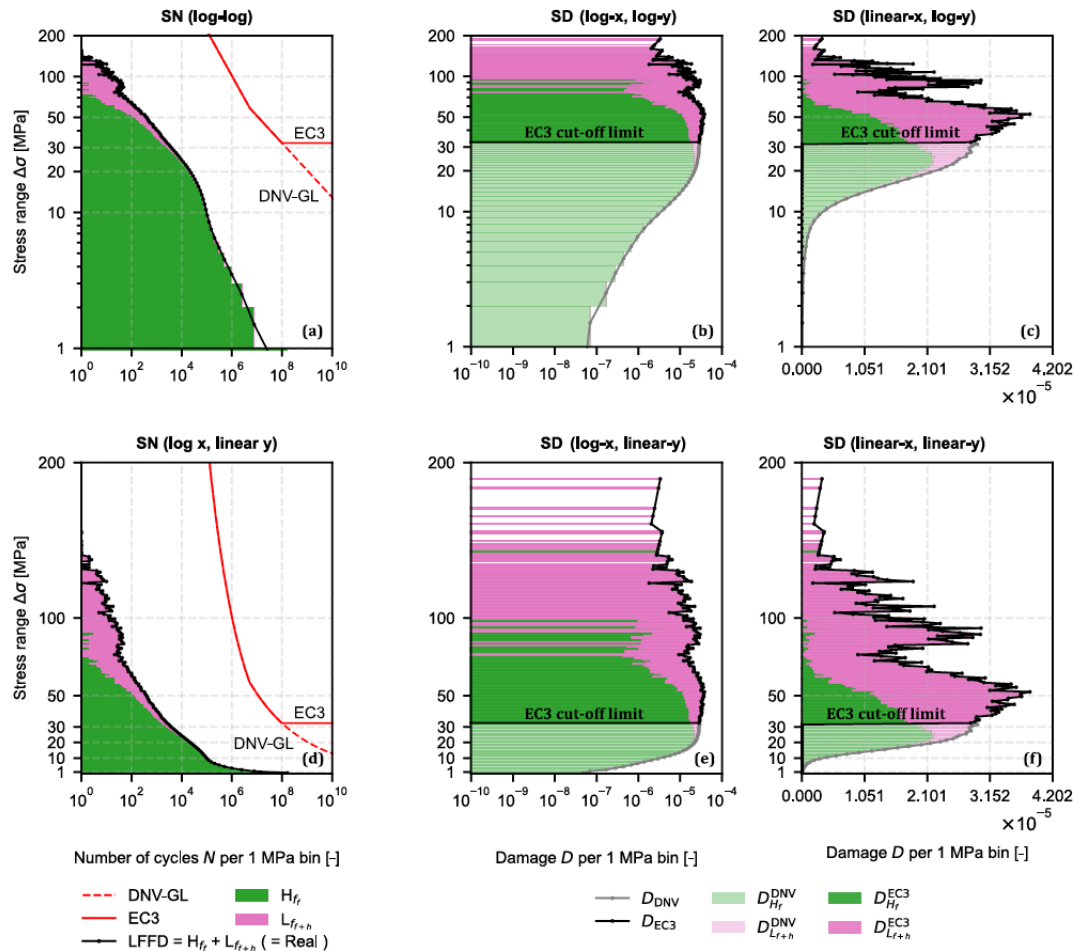
Figure 6. Comparison of \Delta\sigma - N and \Delta\sigma - D fatigue representations for conventional 10 min windows. Panels (a) and (d) show the \Delta\sigma - N distributions together with the EC3 and DNV \sigma - N curves. The top row (a–c) uses logarithmic scaling on the y axis, while the bottom row (d–f) uses linear scaling on the y axis. Panels (b) and (e) present the corresponding \Delta\sigma - D distributions with logarithmic scaling on the x axis, whereas panels (c) and (f) show the same distributions using linear scaling on the x axis. Green and pink denote the LFFD high-frequency and low-frequency fatigue contributions, respectively, while the black curve represents the total fatigue distribution.
