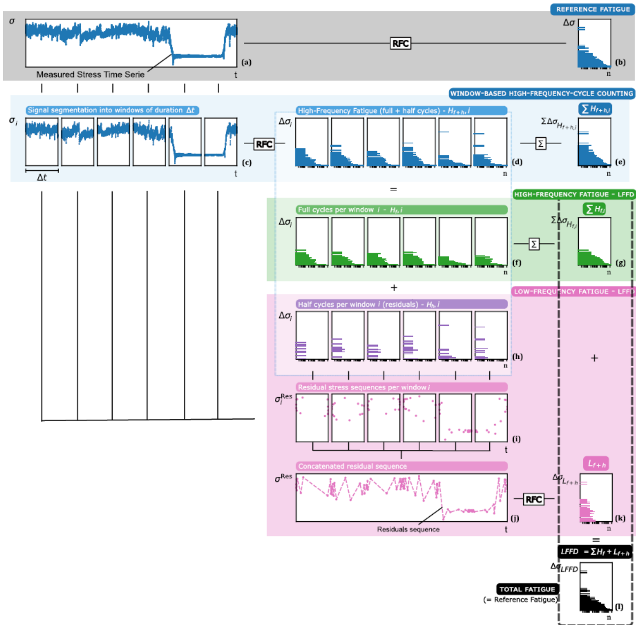
Figure 1. Overview of fatigue monitoring methodologies based on rainflow cycle counting (RFC). (a) Measured stress time series. (b) Base-line fatigue spectrum obtained by applying RFC to the full signal, including full and half cycles. (c) Segmentation of the stress time series into consecutive windows of duration \Delta t . (d) RFC applied independently to each window, yielding window-level fatigue spectra. (e) Aggregated fatigue spectrum obtained by summing full and half cycles across all windows. (f) Full cycles extracted within each window. (g) Aggregated full-cycle spectrum representing the high-frequency, window-contained fatigue contribution. (h) Half cycles remaining in each window. (i) Residual stress sequences associated with unclosed half cycles. (j) Concatenation of residual stress sequences across windows. (k) RFC applied to the concatenated residual sequence, capturing low-frequency fatigue cycles spanning multiple windows. (l) Total fatigue spectrum obtained by combining the high-frequency (full-cycle) and low-frequency (residual-based) contributions, preserving equivalence with continuous RFC.
