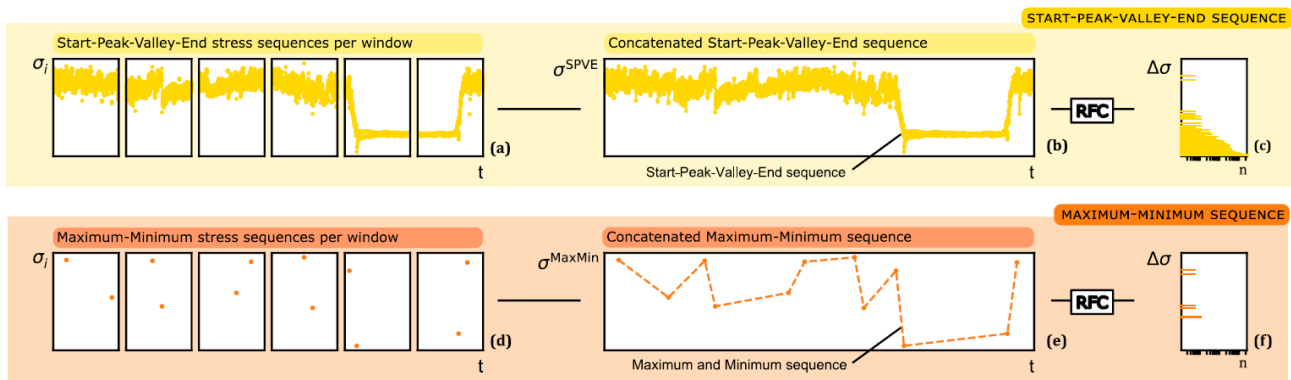
Figure 3. Extrema sequence methods for reduced-information fatigue assessment. (a) Windowed extraction of start, peaks, valleys, and end (SPVE) points within each window. (b) Concatenation of the windowed SPVE values to form a continuous start–peaks–valleys–end sequence; rainflow cycle counting (RFC) is applied to identify fatigue cycles, including those spanning multiple windows. (c) Resulting fatigue spectrum obtained from the SPVE sequence. (d) Windowed extraction of maximum and minimum stress values per window. (e) Concatenation of windowed maxima and minima to form a maximum–minimum (max–min) sequence; rainflow cycle counting (RFC) is applied to identify fatigue cycles. (f) Resulting fatigue spectrum obtained from the max–min sequence. The SPVE approach preserves local turning-point structure, while the max–min approach provides a highly compressed representation emphasising large-amplitude, long-period stress variations.
