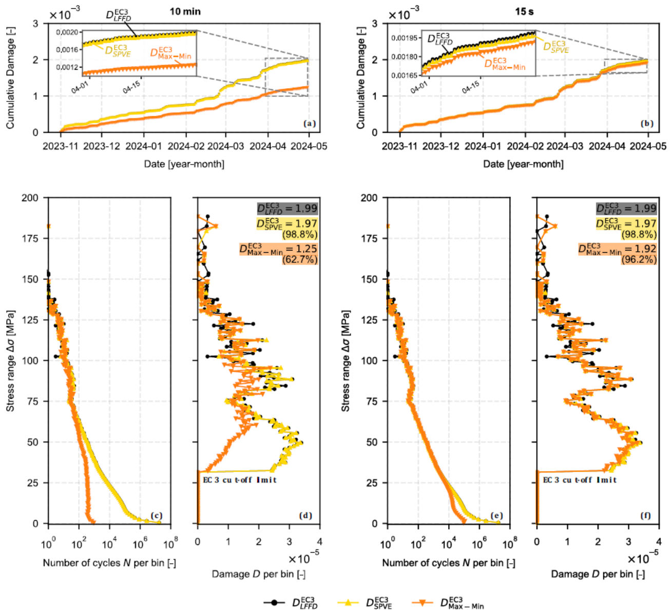
Figure 13. FA-direction fatigue at tower section T1 (6 months, 6.25 Hz): LFFD baseline versus reduced-information extrema representations. (a–b) Cumulative damage for 10 min and 15 s windows. (c, e) \Delta\sigma - N spectra and (d, f) \Delta\sigma - D spectra at the end of the 6 months, for 10 min and 15 s windows respectively. Curves compare LFFD total damage (baseline), start–peaks–valleys–end (SPVE), and maximum–minimum (max–min). Percentages indicate damage relative to the LFFD baseline (Eq. 5, EC3). Insets show a close-up view of the final month of the monitoring period. Damage is computed using EC3 detail category 80, employing a bi-linear formulation with slopes m = 3/5 .
