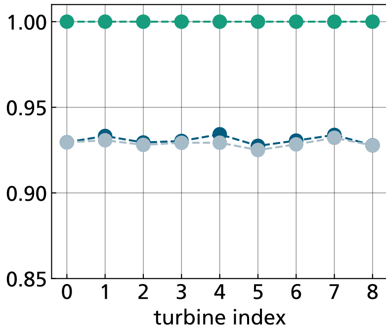
Relative AEP
