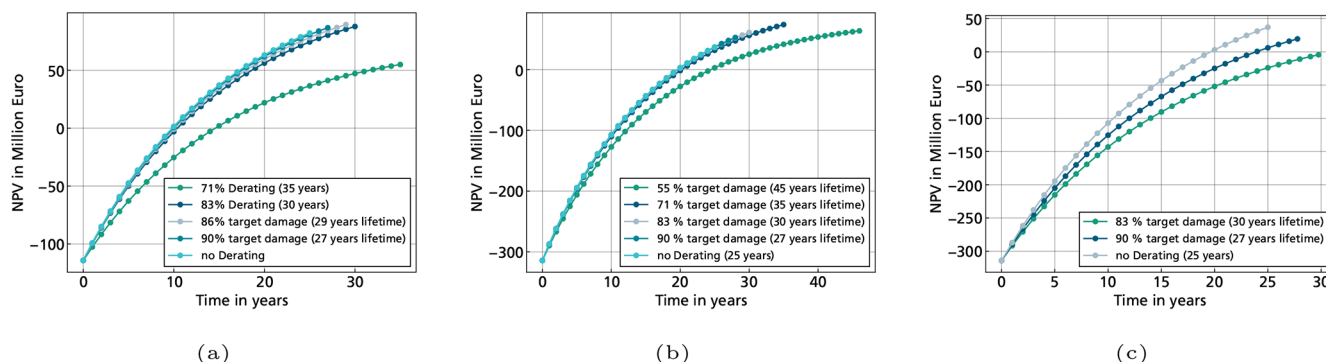
Figure A2. NPV over operating years of the wind farm using the full-farm optimization for case 1 (a), case 2 (b), and case 3 (c).
