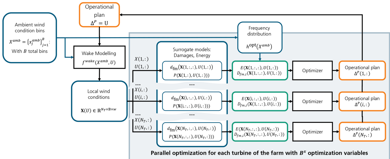
Figure 2. Process for iterative per-turbine optimization.
