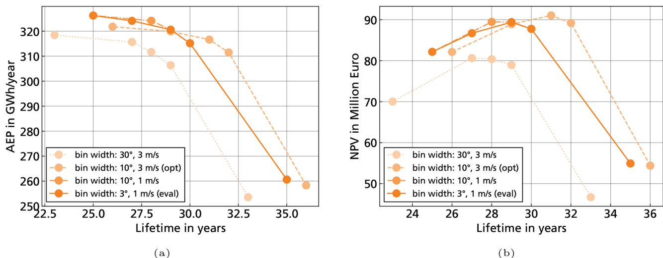
Figure B1. Case 1, onshore scenario with tower as failure mode: comparison of binning sizes of AEP (a) and NPV (b).
