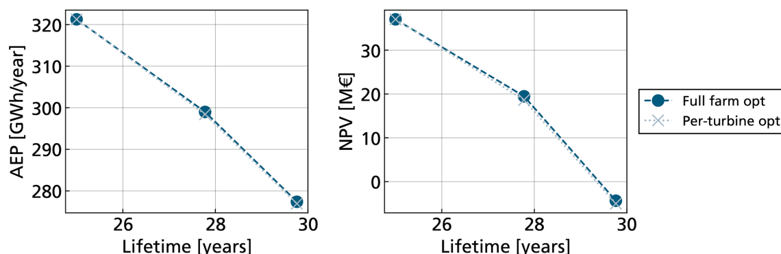
Figure 17. Case 3, evaluation of results: offshore scenario with all failure modes, comparison of AEP and NPV for the optimization approaches.
