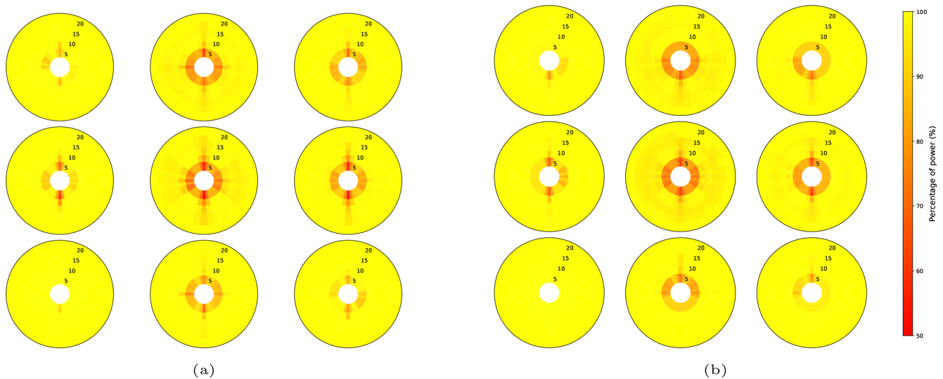
Figure 8. Case 1, onshore scenario with tower as failure mode: optimized operational plan full-farm optimization (a) and per-turbine optimization (b).
