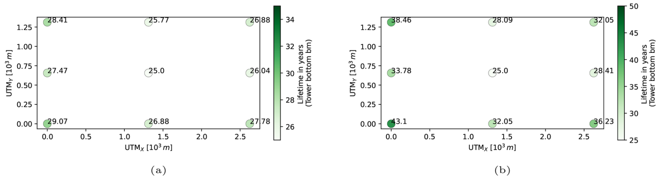
Figure 4. Nominal lifetime (no derating) of the tower bending moment (bm) for the onshore scenario (a) and offshore scenario (b).
