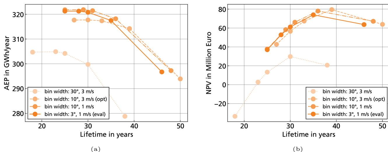
Figure B2. Case 2, offshore scenario with tower as failure mode: comparison of binning sizes of AEP (a) and NPV (b).
