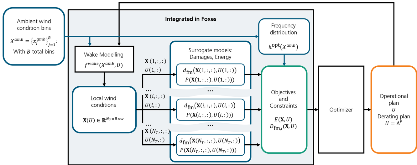
Figure 1. Process for full-farm optimization in single run.
