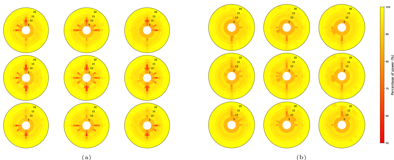
Figure 16. Case 3, offshore scenario with all failure modes: optimized operational plan full-farm optimization (a) and per-turbine optimization (b).
