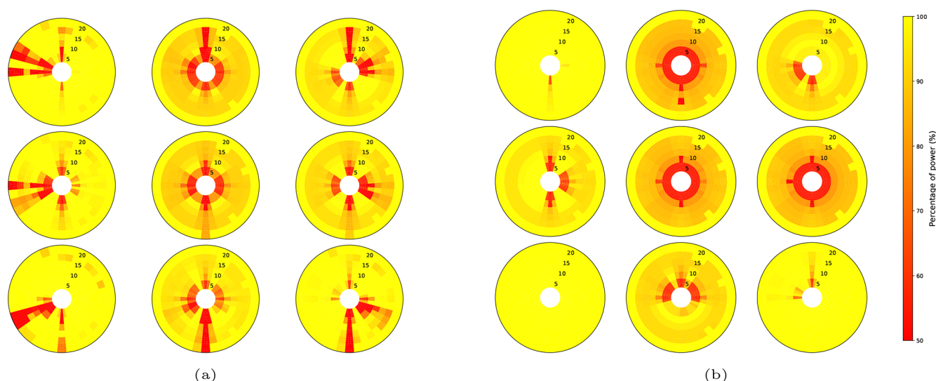
Figure 12. Case 2, offshore scenario balancing tower lifetime at 45 years: optimized operational plan full-farm optimization (a) and per-turbine optimization (b).
