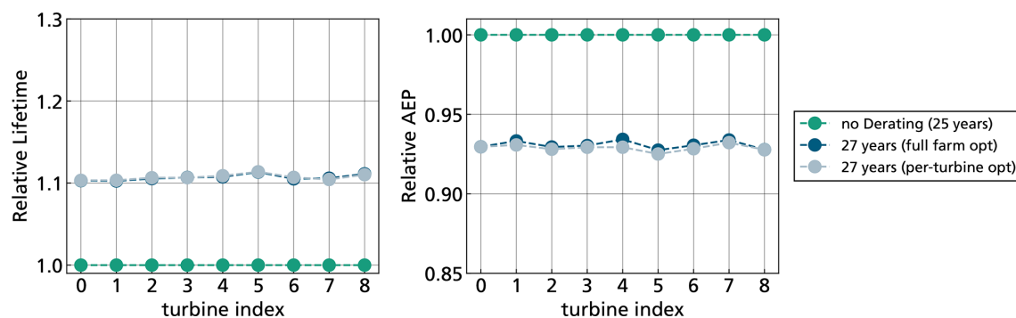
Figure 15. Case 3, offshore scenario with all failure modes: relative values compared to nominal operation (no derating) for lifetime and AEP on each turbine for both optimization methods.
