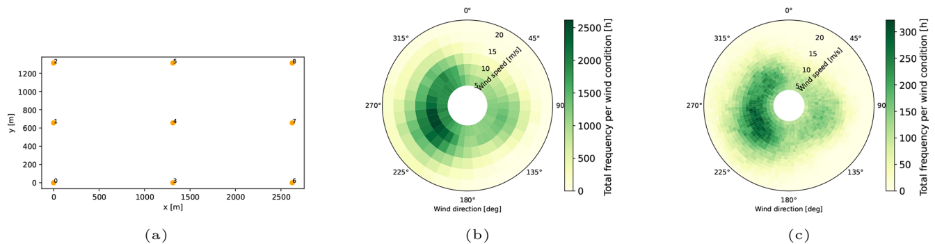
Figure 3. Farm layout with distance in meters; 1 rotor diameter = 164 m (a). Wind distribution given as lifetime frequency for each combination of wind speed and wind direction with broader binning used for optimization h^{\text{opt}} (b) and fine-binning used for evaluation h^{\text{eval}} (c).
