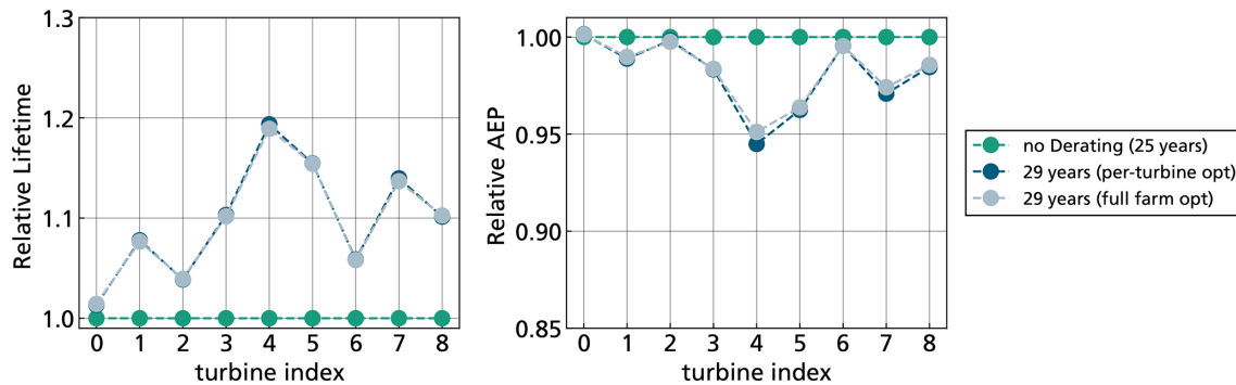
Figure 7. Case 1, onshore scenario balancing tower lifetime at 29 years: relative values compared to nominal operation (no derating) for lifetime and AEP on each turbine for both optimization methods.
