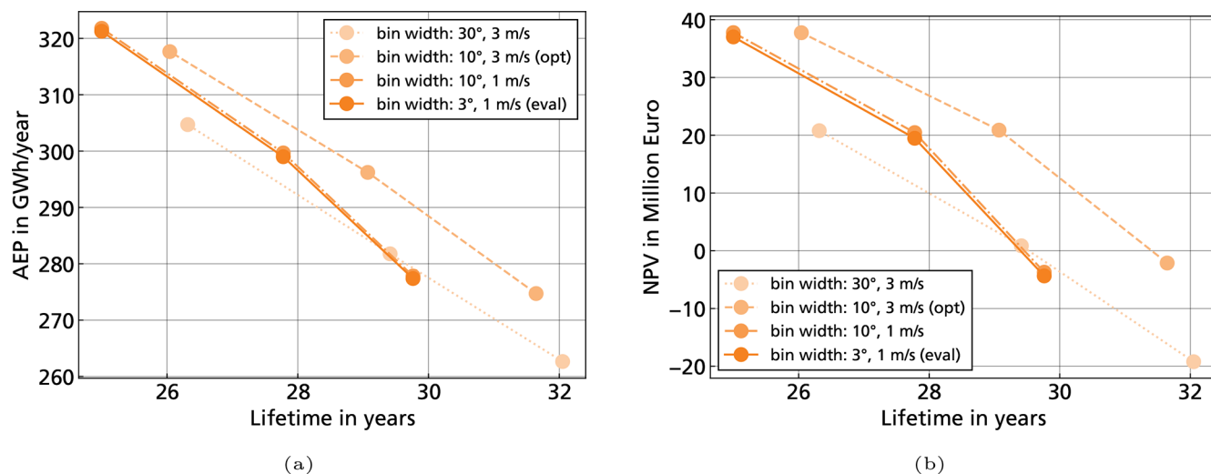
Figure B3. Case 3, offshore scenario with all failure modes: comparison of binning sizes of AEP (a) and NPV (b).
