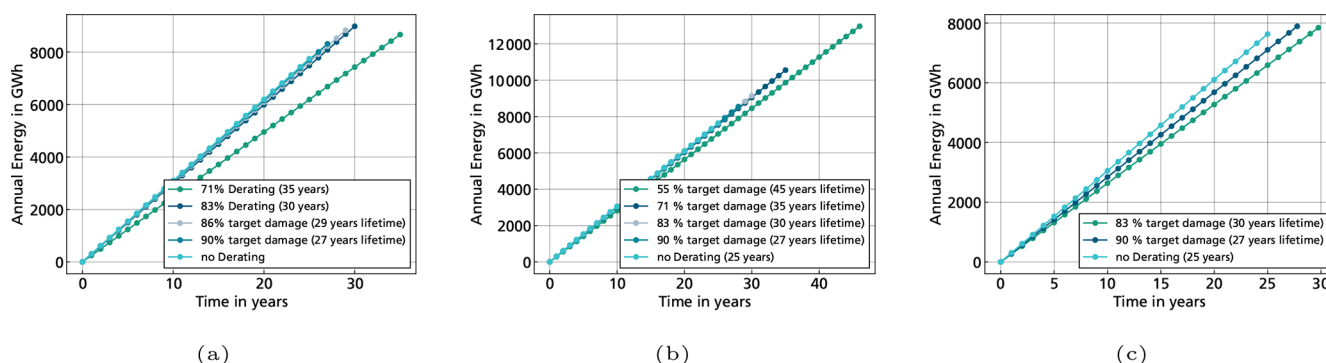
Figure A1. Total energy production over operating years of the wind farm using the full-farm optimization for case 1 (a), case 2 (b), and case 3 (c).
