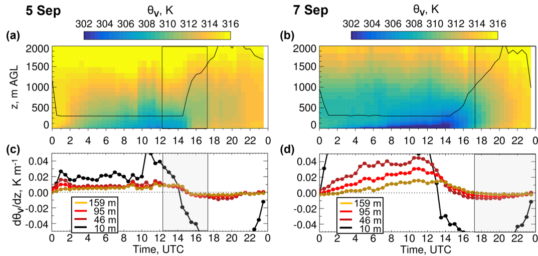
Figure 10. (a) Virtual potential temperature ( \theta_v ) from ASSIST data at Site B on (a) 5 September and (b) 7 September. Black lines show planetary boundary layer height (m) derived from the retrieved fields. Virtual potential temperature gradient ( d\theta_v/dz ) on (c) 5 September and (d) 7 September at 10 m a.g.l. and three heights within the limits of turbine blades. Shaded gray areas indicate periods of PUMAS measurement on each day.
