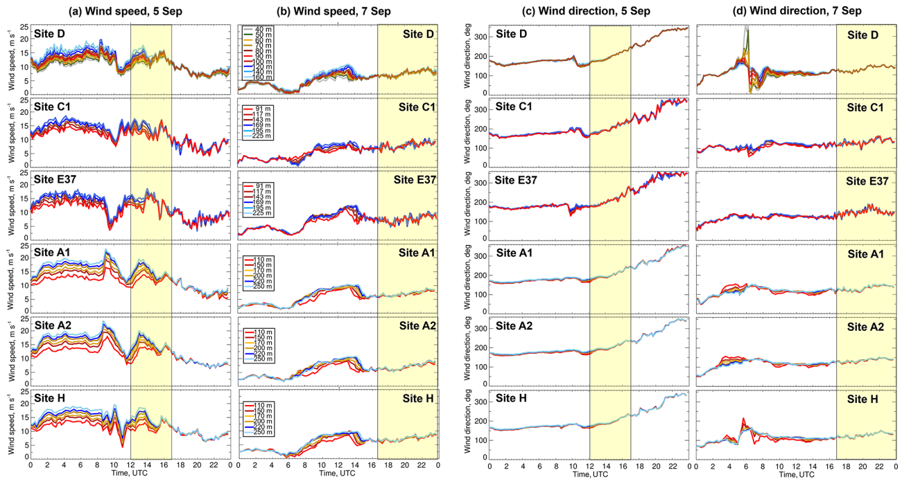
Figure 9. Time series of (a, b) wind speed and (c, d) wind direction from six stationary Doppler lidars at lowest heights on 5 and 7 September. Locations of lidar sites (Site D, Site C1, Site E37, Site A1, Site A2, and Site H) are shown in Fig. 4. The heights of measurements are indicated in the legend for each lidar. Periods of PUMAS operations on 5 and 7 September are highlighted in yellow.
