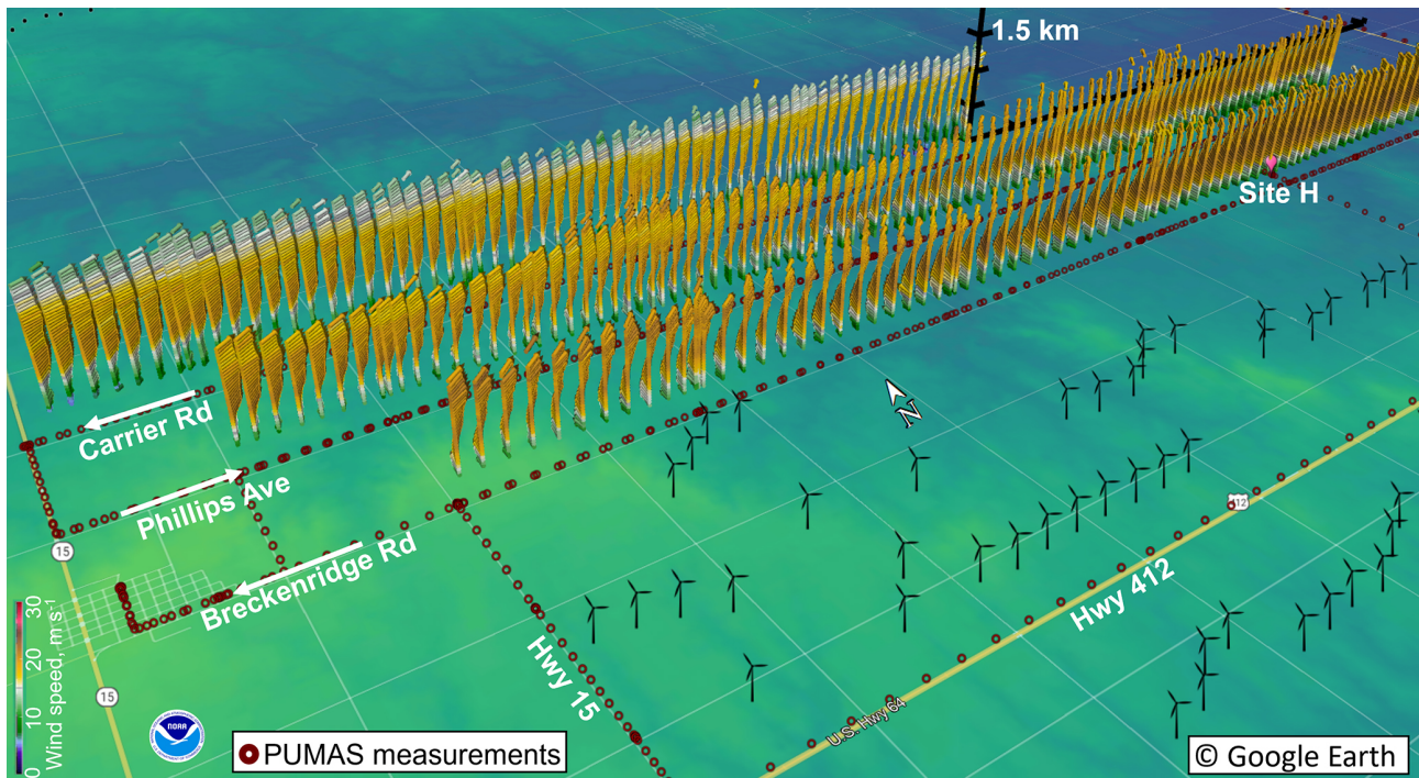
Figure 17. Wind speed (colors) and direction (arrows) profiles on 5 September are shown along individual transects on Breckenridge Rd. (13:14–13:34 UTC), Phillips Ave. (13:52–14:14 UTC), and Carrier Rd. (14:37–14:51 UTC) selected for the analysis. The dark-red circles indicate points of PUMAS measurements on 5 September. Profiles are embedded on a Google Earth terrain elevation map (Debnath et al., 2022) and rotated clockwise \sim 60^\circ for a better view. Wind speed is scaled from 0 to 30 \text{ m s}^{-1} according to the color scale on the left side of this figure. The horizontal distance between profiles is about 300 m. White arrows in the left corner indicate the PUMAS driving direction for each transect in this example. Figure 17 is created using map data © Google Earth 2023.
