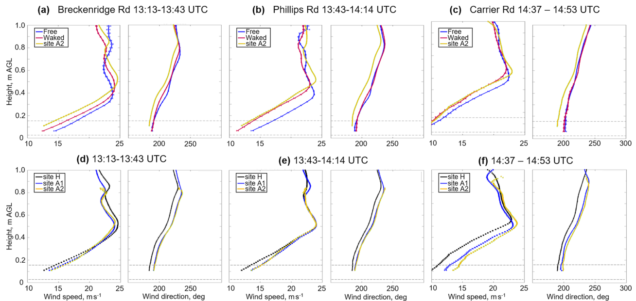
Figure 19. Similar to Fig. 14 but for the mean profiles during transects on 5 September shown in Fig. 17.
