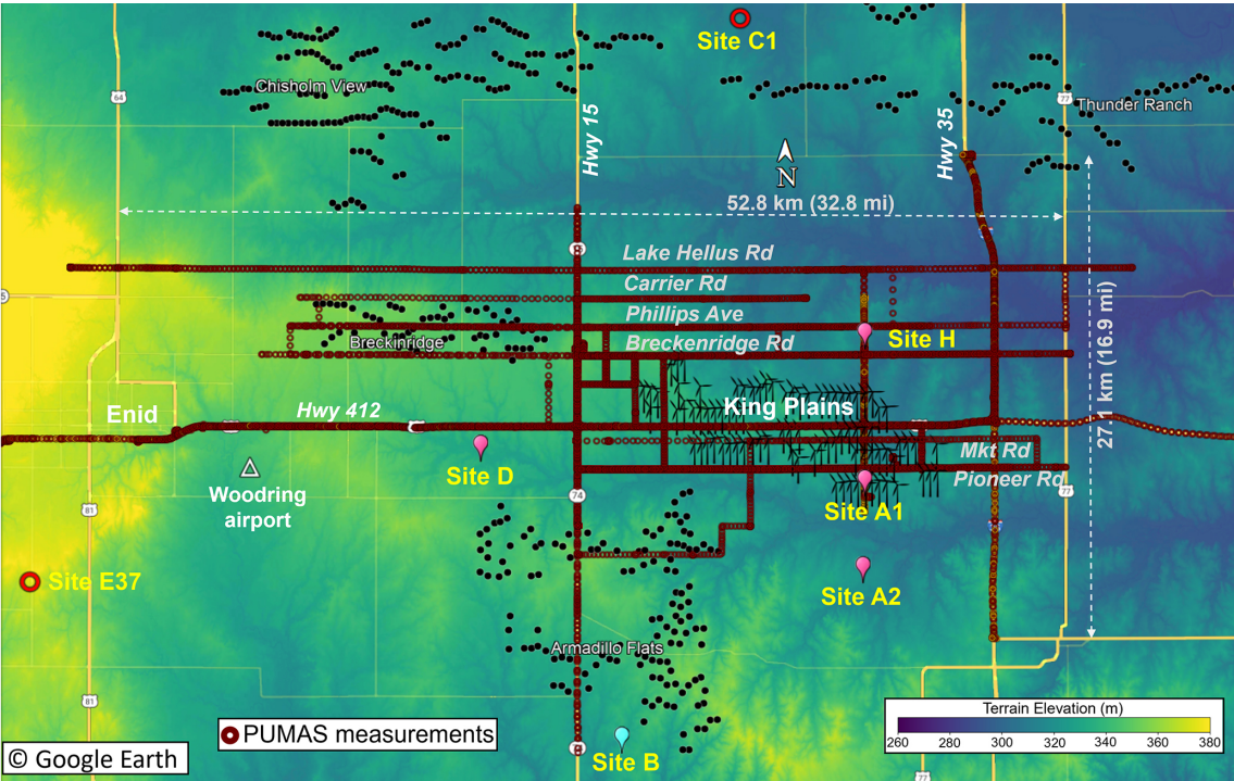
Figure 3. Wind farms in northern central Oklahoma are shown on the terrain elevation map (Debnath et al., 2022) by black dots. Turbine symbols show King Plains wind farm to underline the research focus on this area. Red circles indicate the ARM SGP highly instrumented Central Facility C1 and the extended facility E37 ( https://www.arm.gov/capabilities/observatories/sgp , last access: 12 November 2024). Pink and cyan pins indicate AWAKEN lidar and ASSIST sites used in this paper. The roads (transects), covered by PUMAS during AWAKEN, are shown by dark-red circles where each circle represents a profile measurement from 64 m up to several kilometers a.g.l. The white triangle indicates the Woodring Regional Airport in Oklahoma, located about 8 km southeast of the central business district of Enid, Oklahoma. This figure is created using map data © Google Earth 2023.
