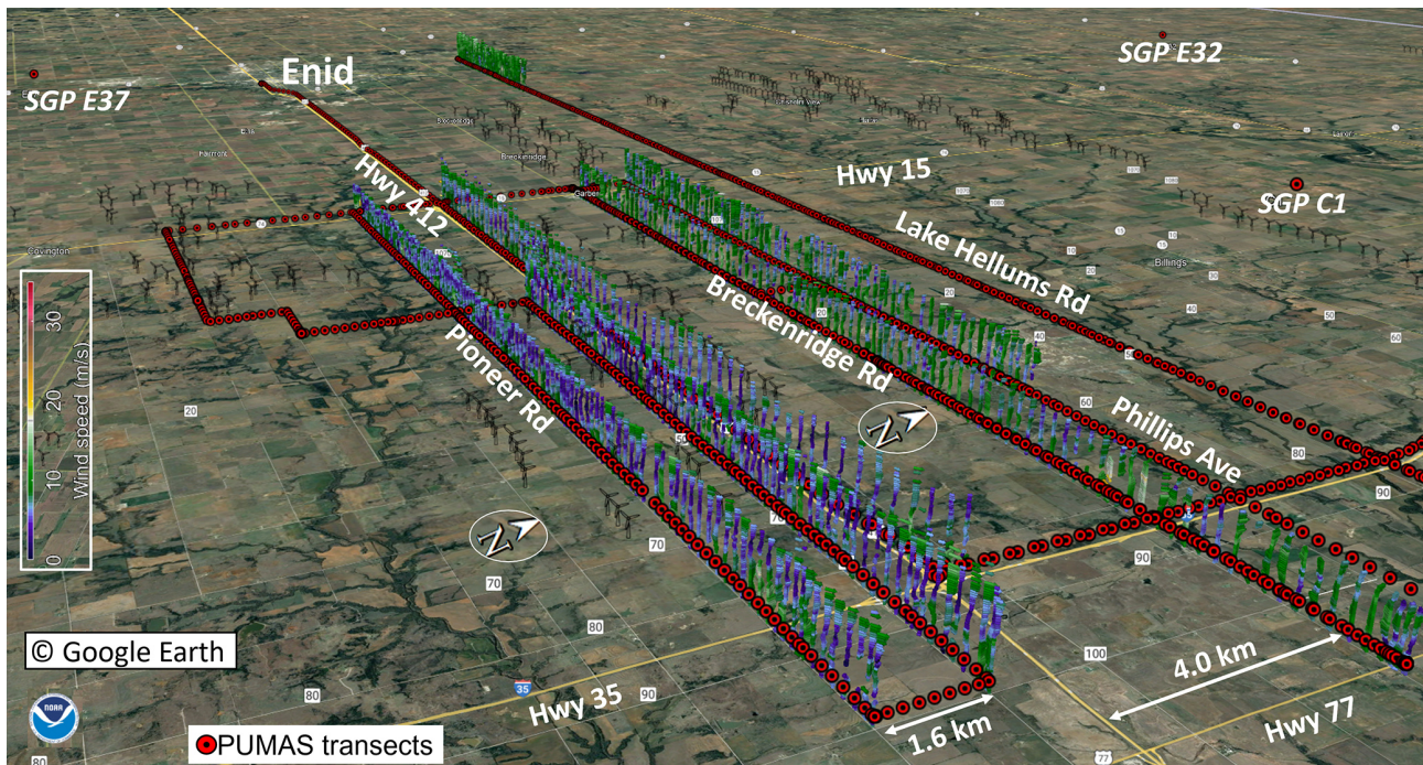
Figure 12. Samples of wind profiles along some transects on 5 September 2023, embedded on Google Earth, are rotated clockwise \sim 45^\circ for a better view. Profiles are shown up to 1.5 km a.g.l., and wind speed is scaled from 0 to 30 \text{ m s}^{-1} according to the color scale on the left side of this figure. The horizontal distance between profiles is about 300 m. White arrows indicate distances between illustrated transects along the named roads. Gray circles indicate the ARM SGP sites (C1, E37, and E32). Figure 12 is created using map data © Google Earth 2023.
