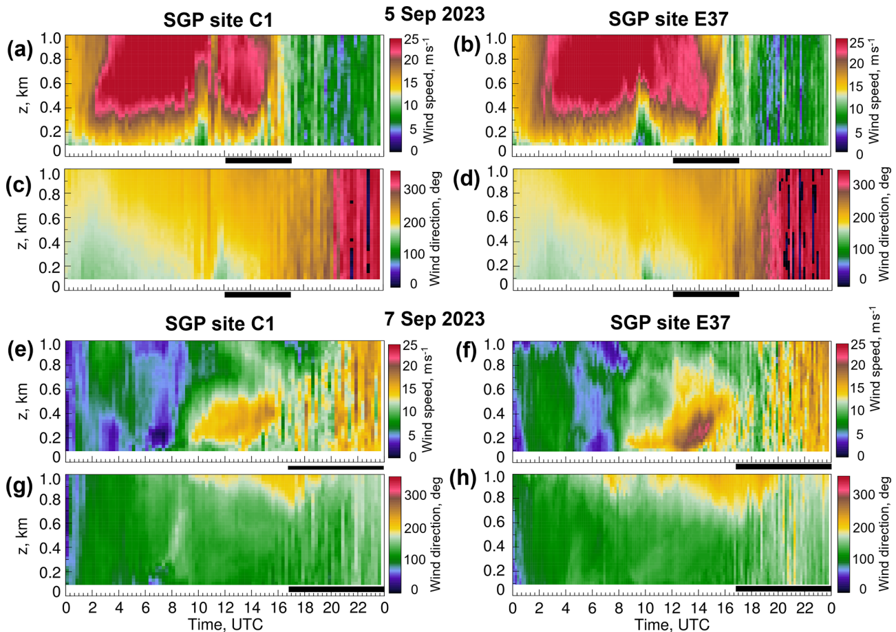
Figure 8. Time–height cross-sections of wind speed and wind direction from stationary lidar measurements at the SGP sites C1 (left) and E37 (right) on (a–d) 5 September and (e–h) 7 September 2023. Black lines indicate periods of PUMAS measurements on these days. The temporal resolution of lidar data at C1 is 15 min, and that at E37 is 10 min. Lidar data at SGP sites can be found in the DOE ARM archive (Shippert et al., 2010, 2016).
