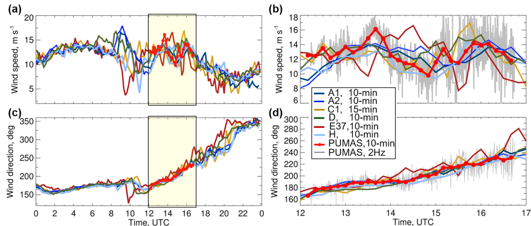
Figure 16. Wind speed and wind direction at 90–110 m from several AWAKEN stationary Doppler lidars and PUMAS on 5 September 2023: (a) time series of 10 min (15 min at C1) data from stationary lidars at several sites are shown for 24 h by colors according to the color scale. Data are taken close to the hub height: 90 m at sites C1, E37, D, and PUMAS; 110 m at sites A1, A2, and H. Yellow boxes indicate the time of PUMAS measurements on this day. (b) Same as panel (a) but for the period of PUMAS measurements at 12:00–17:00 UTC. Gray indicates 2 Hz PUMAS, and the red line with dots shows 10 min averages.
