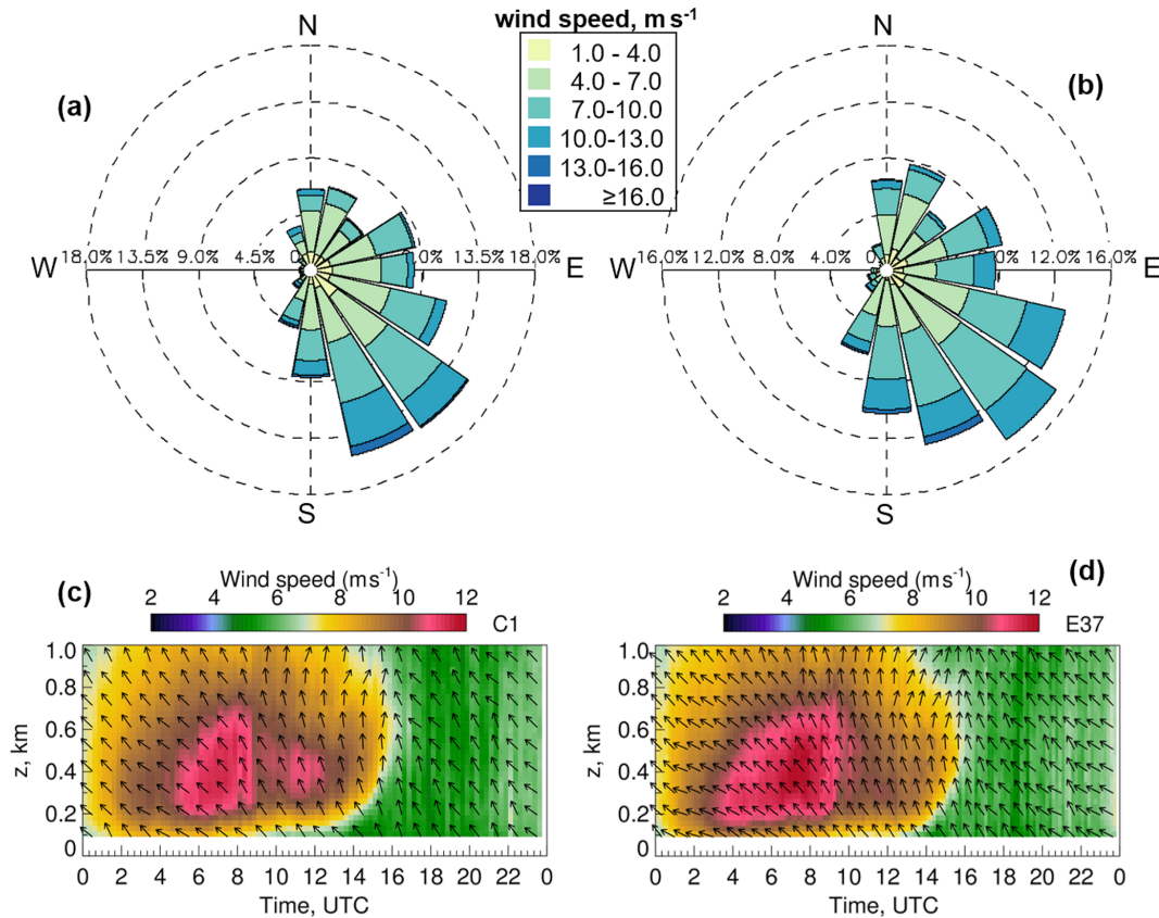
Figure 4. Wind roses of 91 m winds from Doppler lidars at the ARM SGP sites (a) C1 and (b) E37 for all hours of measurements during 15 August–12 September 2023. (c, d) Time–height cross-sections of period-mean wind speed (colors) and wind direction (arrows) from each Doppler lidar. Local time = UTC–5.
