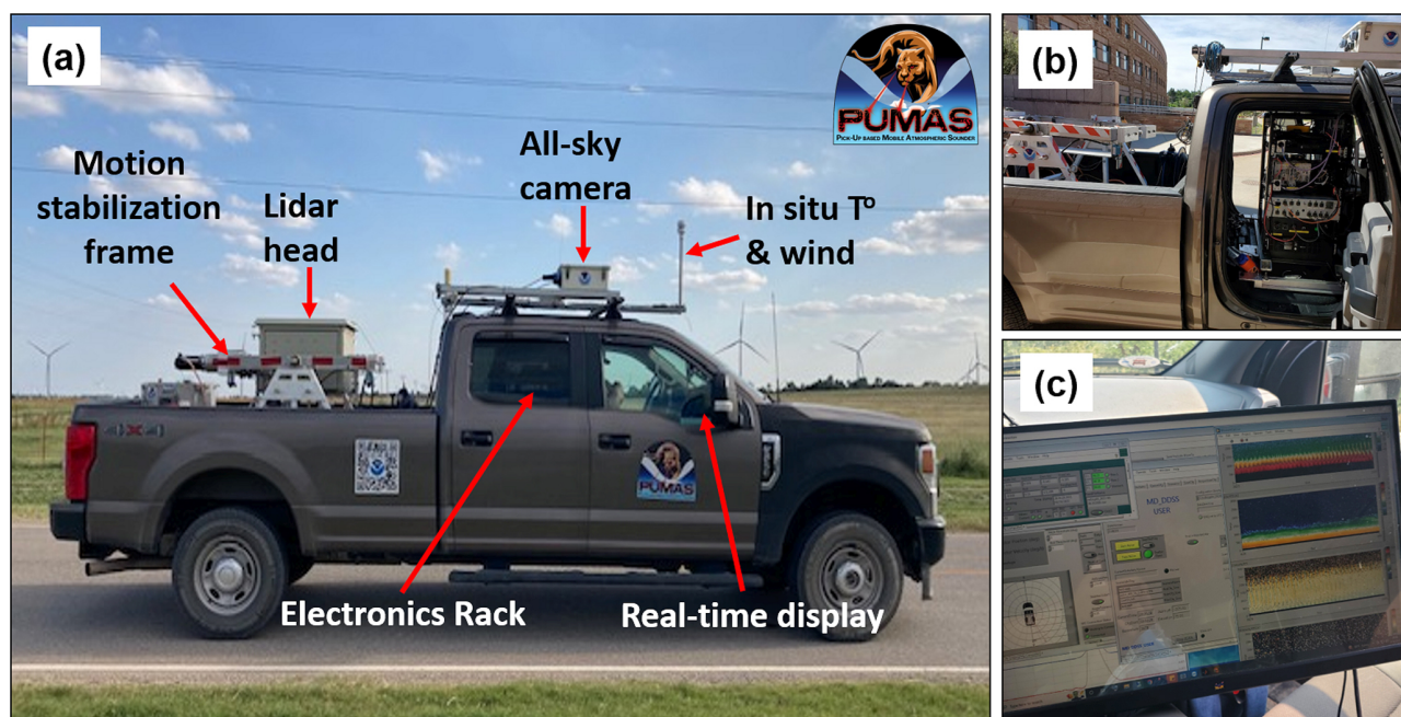
Figure 2. (a) Picture of PUMAS with indicated subsystems: motion-stabilization frame, lidar head, all-sky camera, and the sensor for in situ measurements of temperature ( T^\circ ) and wind speed; (b) the electronics rack located in the back of a cabin; (c) real-time display located in the front of the cabin.
