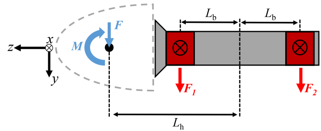
Figure 2. Force diagram of a main shaft in a four-point support drivetrain. Note that the z axis is aligned with the turbine drivetrain and hence sits at a tilt angle relative to the ground. Force and moment vector components (including the definition of “positive direction”) at each location are defined via the depicted HAWC2 reference frame.
