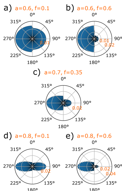
Figure 4. Edge case wind direction roses, in terms of a and f values, are shown in subplots (a), (b), (d), and (e). The full envelope of applied wind direction roses fell between these bounding cases, each with a prevailing wind direction of 270^\circ . The “median” wind rose, i.e. with a and f values at the centre of each variable’s range, is shown in subplot (c).
