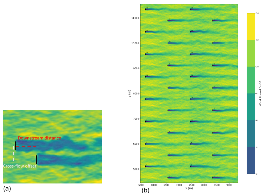
Figure 3. Layouts considered in this study. (a) A snapshot of the two-turbine parametric analysis. The downstream distance was held at 5D , and the cross-flow offset distance between the turbines varied. Note that a negative cross-flow offset is shown in the figure. (b) Layout and flow-field visualization of the TotalControl 32-turbine reference wind farm (Andersen et al., 2018), including wake effects. Turbine indexes are also given.
