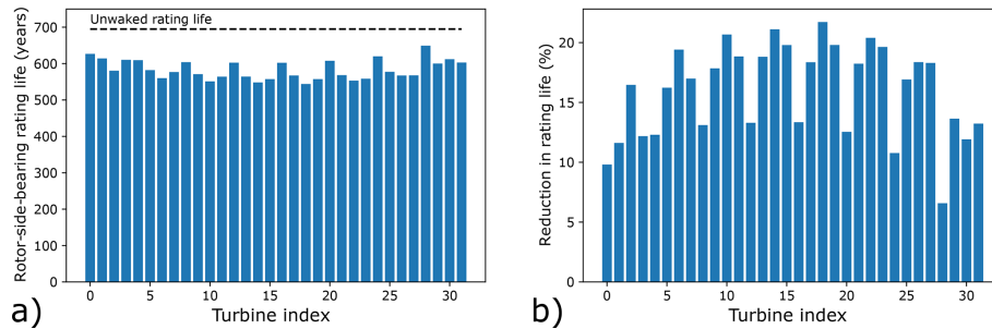
Figure 6. (a) Rating life results for all rotor-side main bearings, obtained from a wind direction rose with parameters a = 0.7 and f = 0.35 . The rating life corresponding to unwaked operation is also shown. (b) Percentage reductions in rotor-side main bearing rating lives, for the same wind rose, relative to the unwaked rating life.
