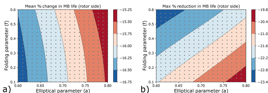
Figure 7. (a) Mean percentage change in rotor-side main bearing rating lives (relative to the unwaked case) across the wind farm, as a function of wind direction rose parameters. (b) Maximum percentage reduction in rotor-side main bearing rating life (relative to the unwaked case) observed within the wind farm, as a function of wind direction rose parameters. The grey dots indicate the parameter combinations considered and therefore the data locations used to determine the resulting contours.
