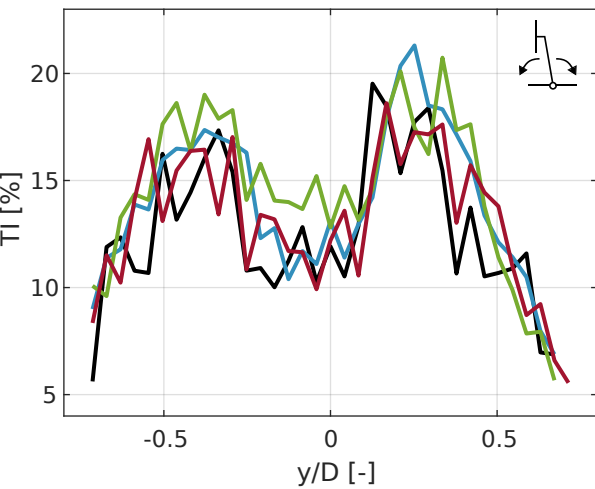
ALM URANS UNIFI
