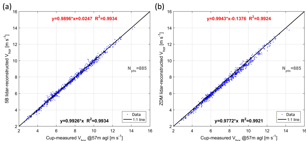
Figure 10. Comparison between mast-measured and lidar-estimated horizontal wind speed at 57.5 m height a.g.l. and 2.5D_{rot} using short-range measurements. (a) 5B-Demo lidar, using five LOS and four ranges. (b) ZDM lidar, using six LOS and three ranges.
