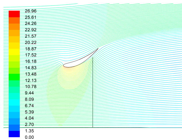
Figure 11. Streamlines of design for optimal C_{p,total} .
