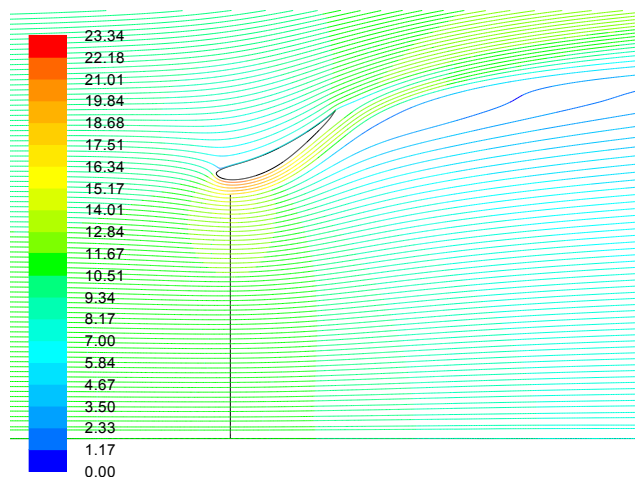
Figure 7. Streamlines of design for optimal C_p .
