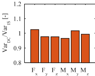
Tower bottom loads
