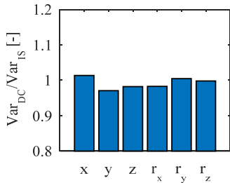
Tower top displacement
