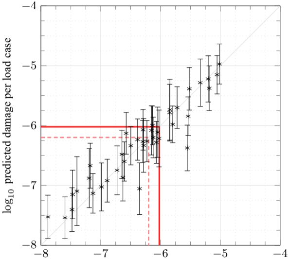
(a) \log_{10} calculated damage per load case
