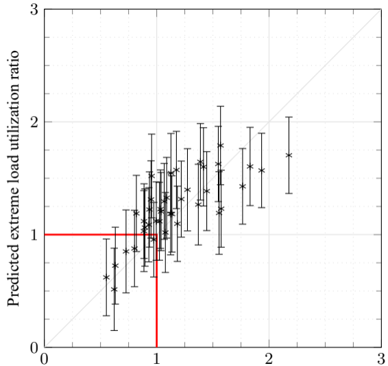
(b) Calculated extreme load utilization ratio
