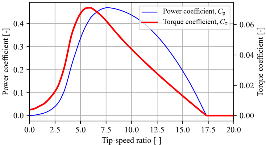
Rotor power and torque coefficient at fine-pitch
