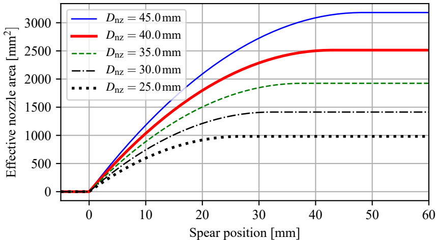
Effective nozzle area for different nozzle diameters
