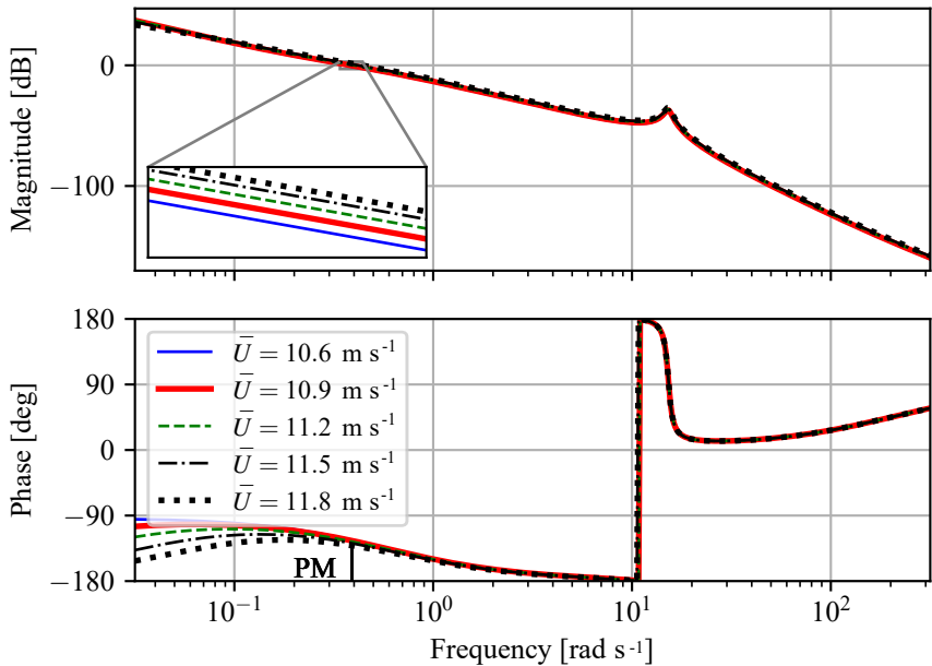
Bode loop transfer w/o k_{s,Q_w} , in: e_s out: \omega_r
