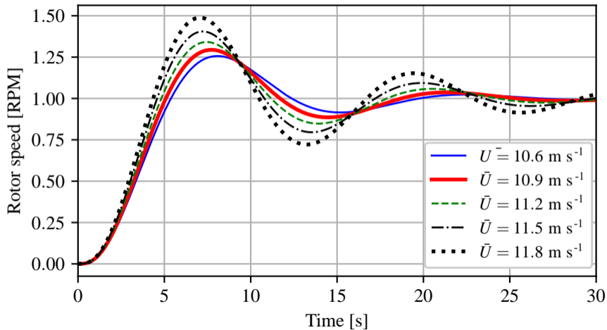
Closed-loop step response, in: \omega_{r,s} out: \omega_r
