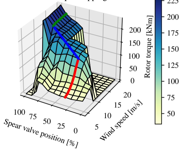
Rotor torque mapping
