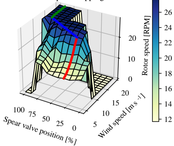
Rotor speed mapping
