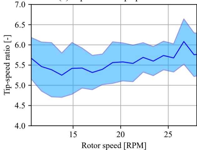
(b) Operational tip-speed ratio
