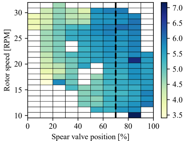
(a) Tip-speed ratio mapping
