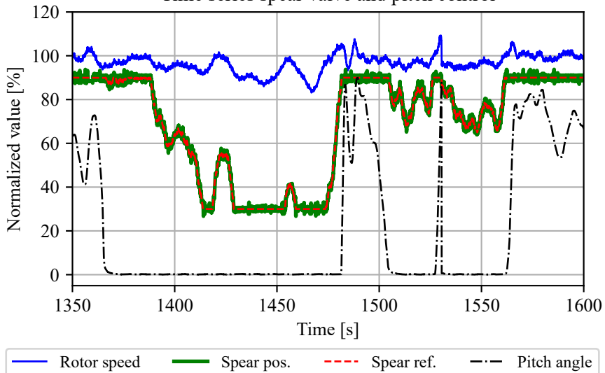
Time series spear valve and pitch control
