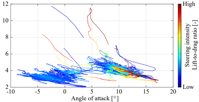
Lift-to-drag ratio [-]
