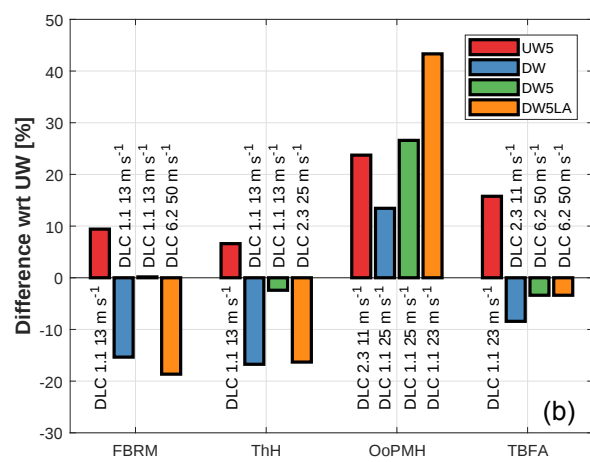
(b) Ultimate loads and corresponding DLC.
