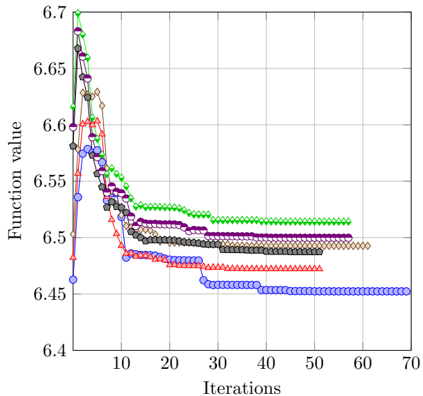
Interior point
