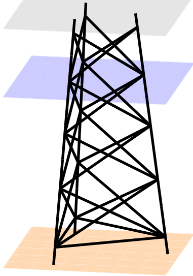
Three-legged jacket with four bays
