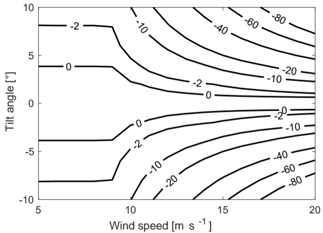
(b) Power difference [%]
