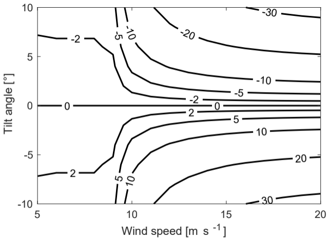
(a) Equilibrium yaw angle [°]
