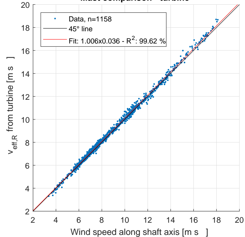
Mast comparison - turbine
