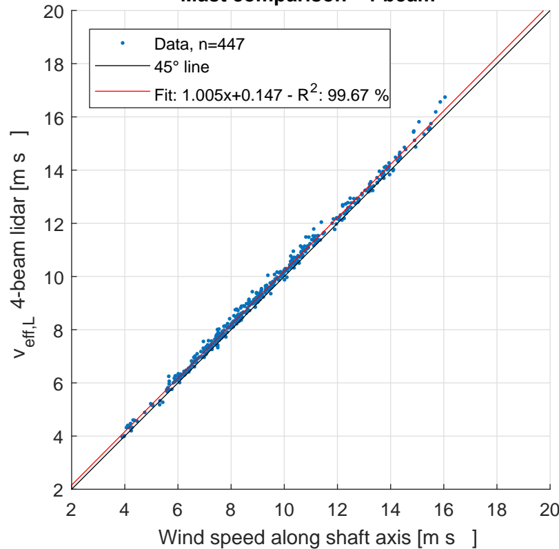
Mast comparison - 4-beam
