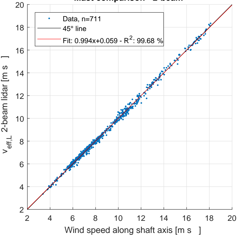
Mast comparison - 2-beam
