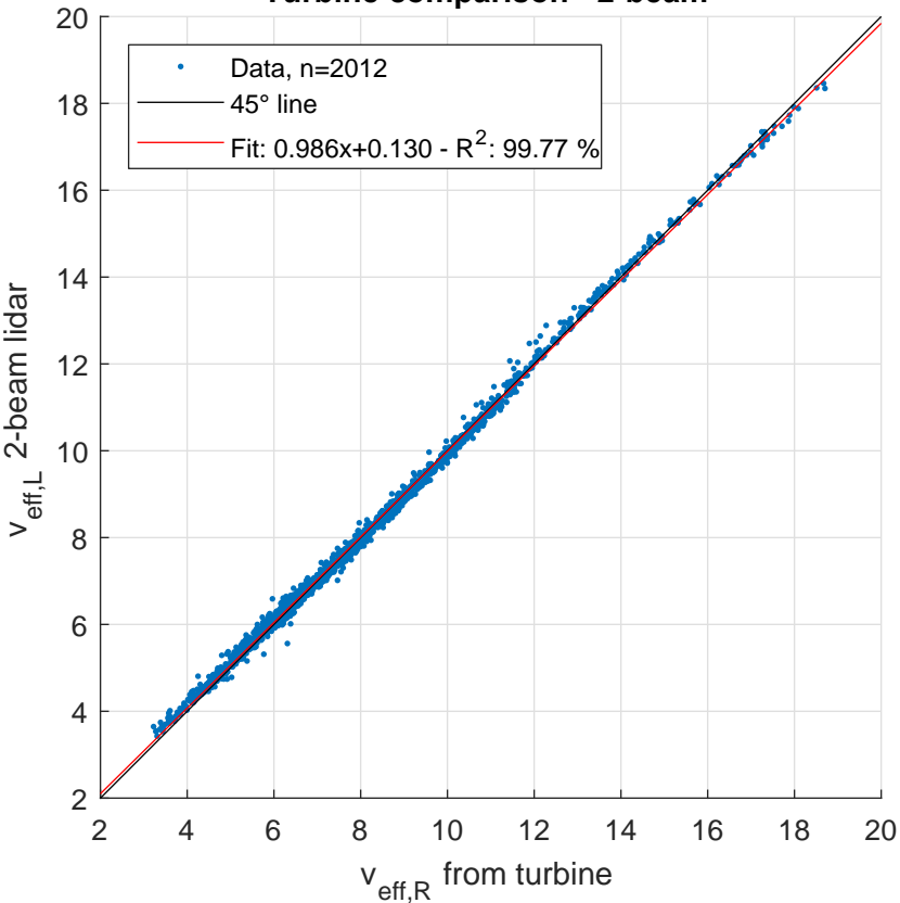
Turbine comparison - 2-beam
