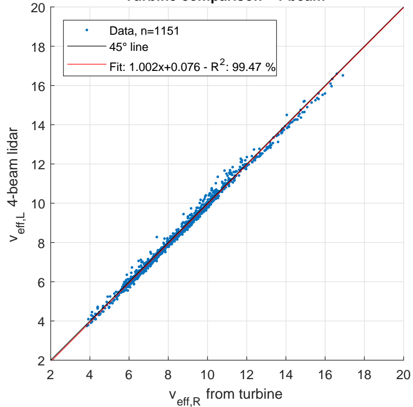
Turbine comparison - 4-beam
