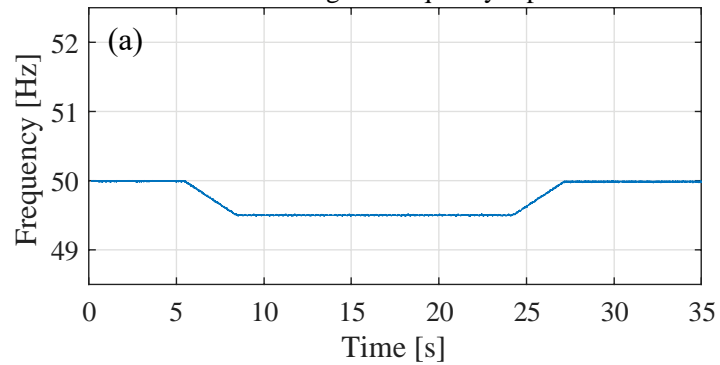
Testing for frequency dip
