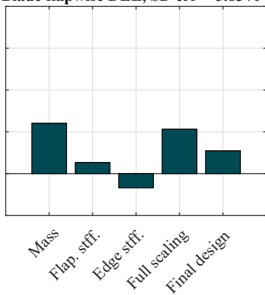
Blade flapwise DEL, SD err = 5.83%
