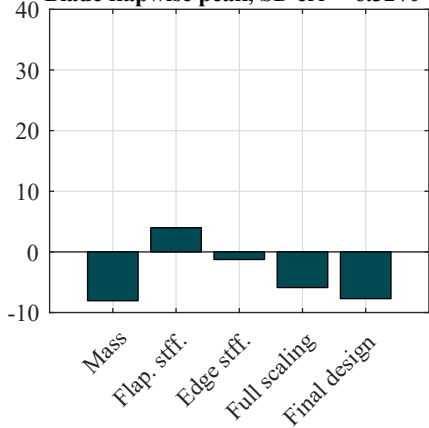
Blade flapwise peak, SD err = 6.32%
