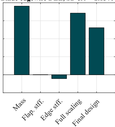
Blade edgewise DEL, SD err = 2.15%
