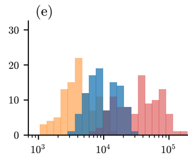
Function calls
