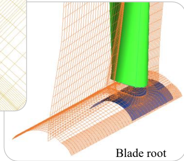
Blade grid
