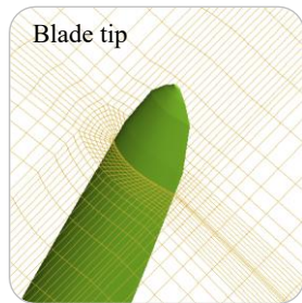
Blade grid
