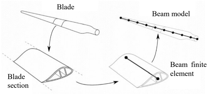
Equivalent beam model (Branner, 2012)
