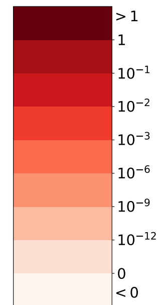
Constraint violation
