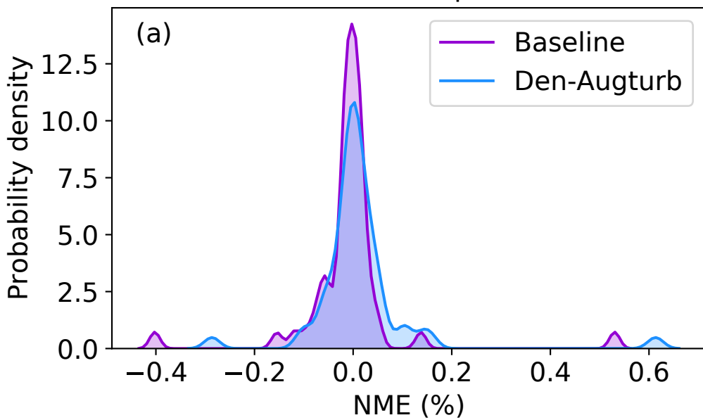
Normalized wind speed: 0-0.1
