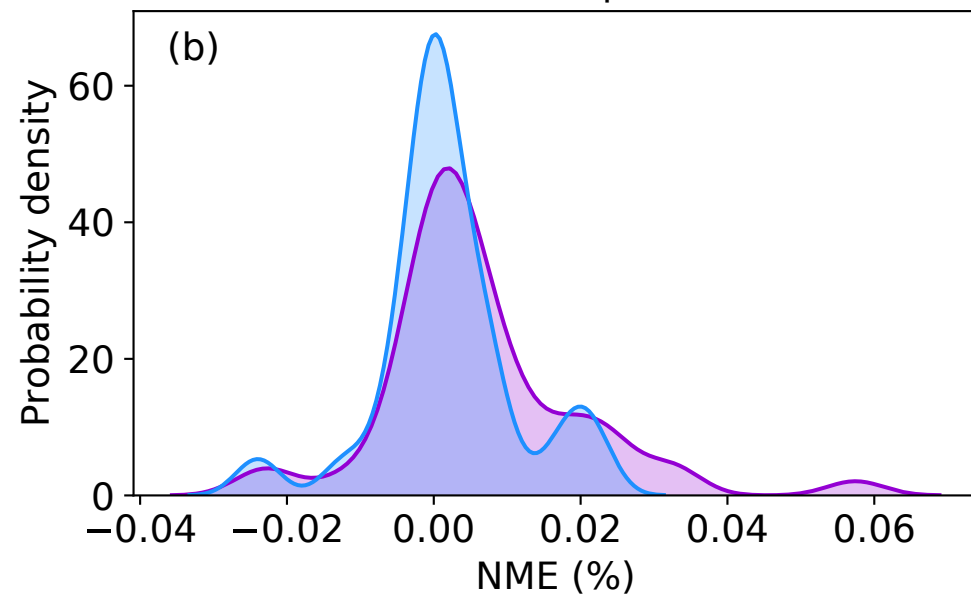
Normalized wind speed: 1.4-1.5
