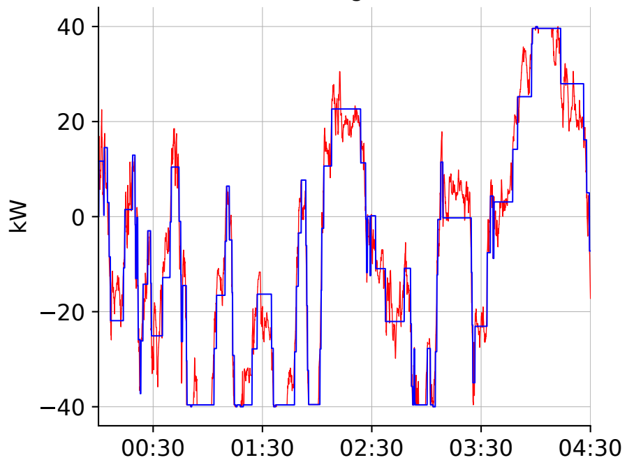
(b) - 4.5 h AGC signal (Test 3)
