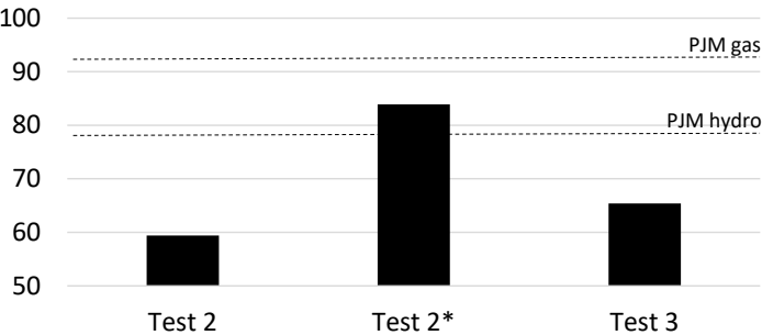
(b) PJM \eta (%)
