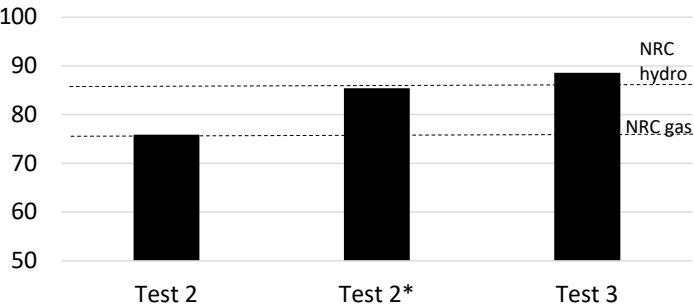
(a) NRC \eta (%)
