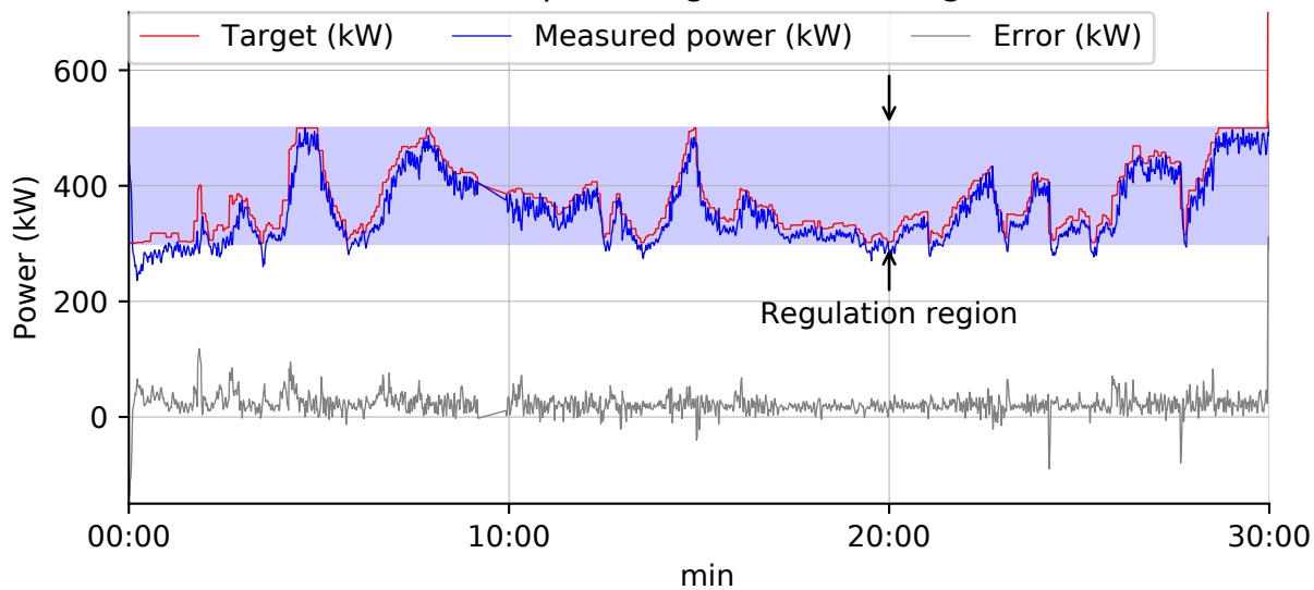
(b) - Turbine providing 100 kW of regulation
