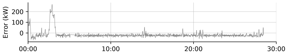
(b) - Turbine providing 100 kW of regulation
