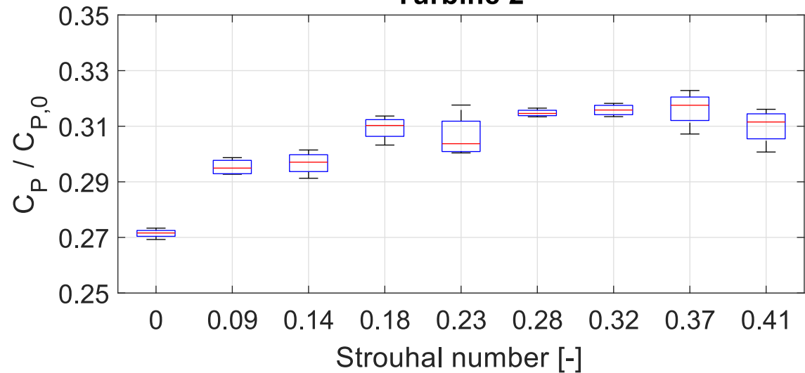
Turbine 2
