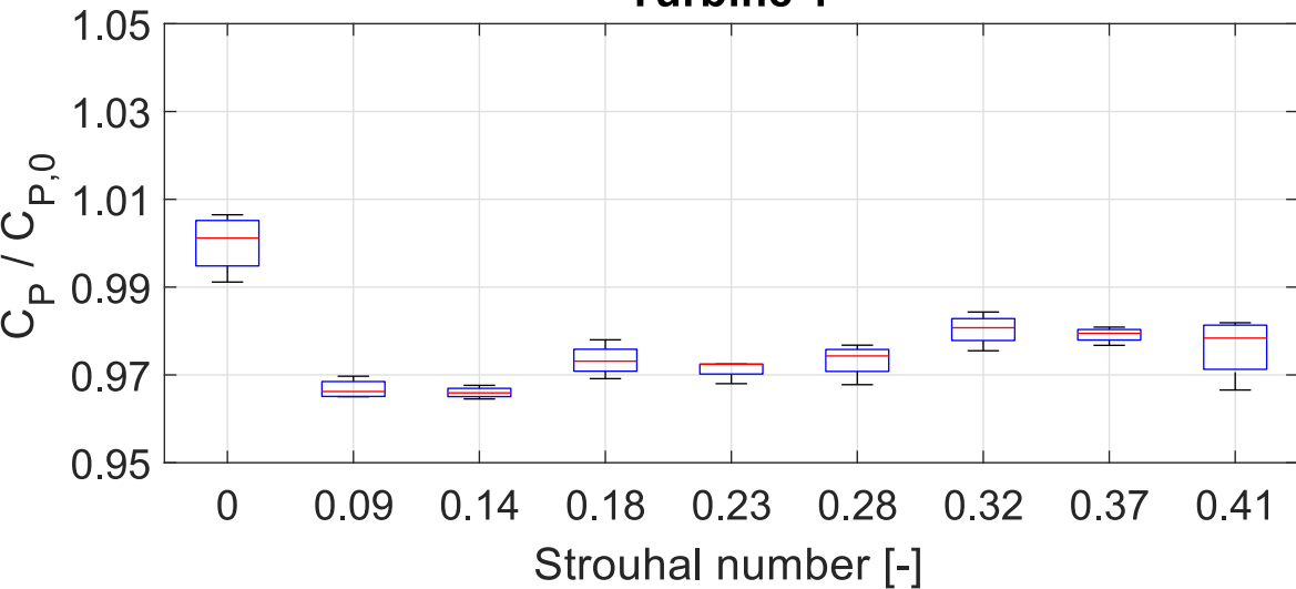
Turbine 1
