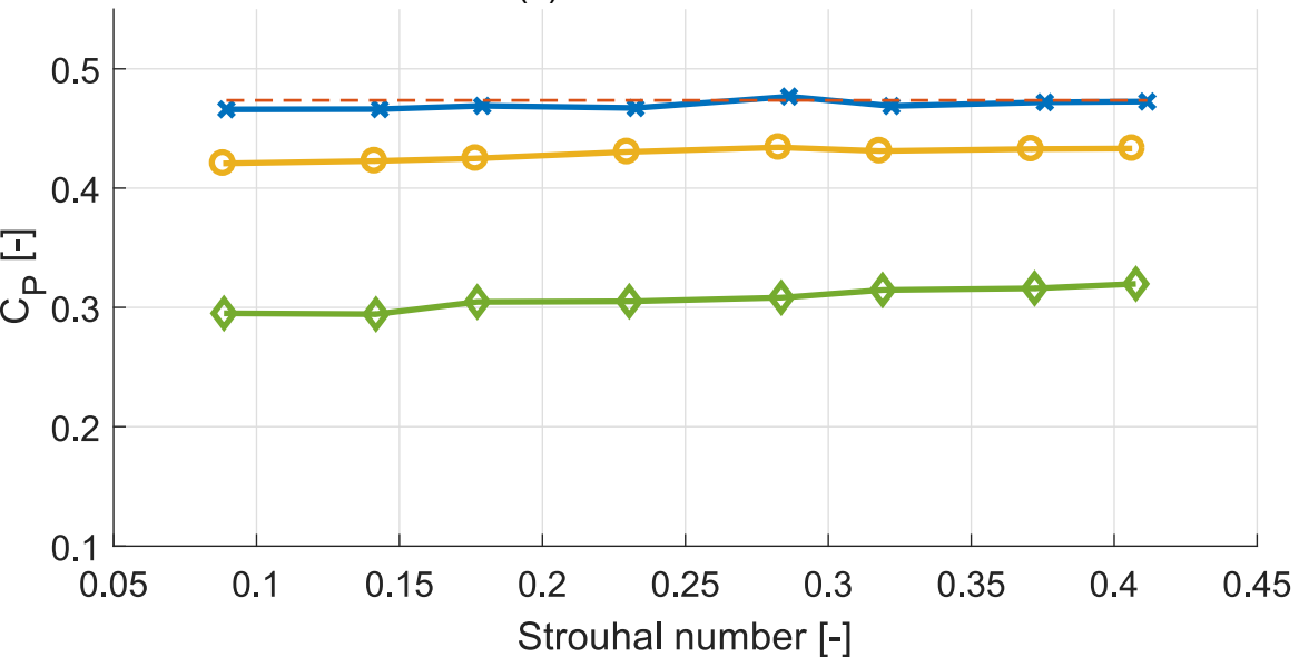
(a) Turbine 1
