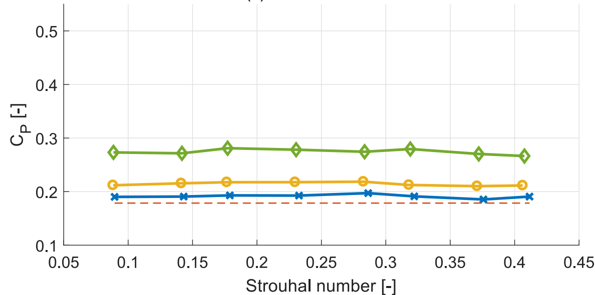
(b) Turbine 2
