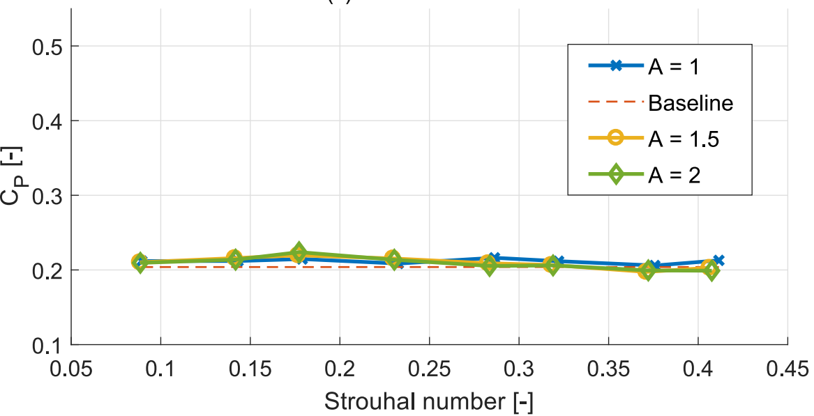
(c) Turbine 3
