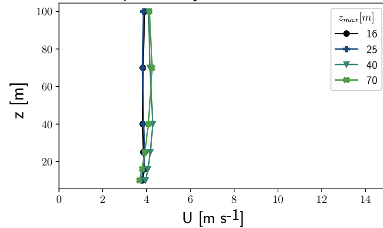
Skipheia, very unstable conditions
