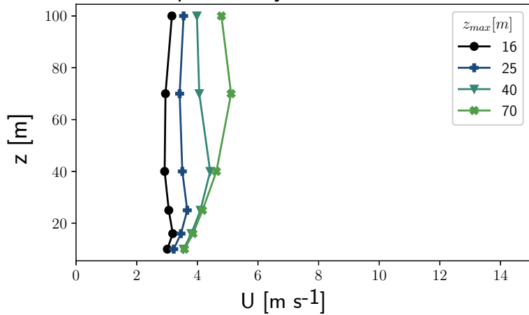
Skipheia, very stable conditions
