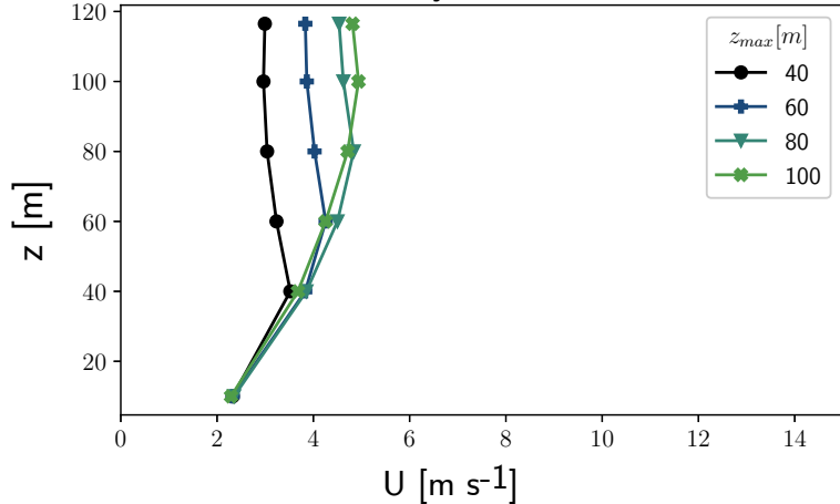
Høvsøre, very stable conditions
