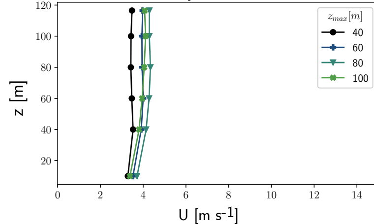
Høvsøre, very unstable conditions
