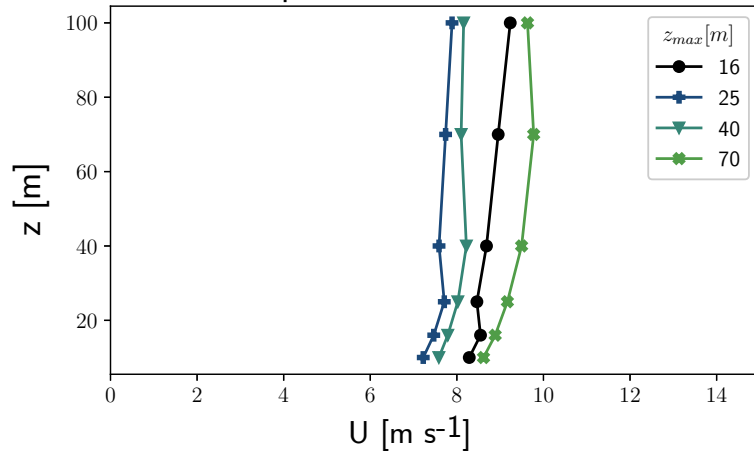
Skipheia, neutral conditions
