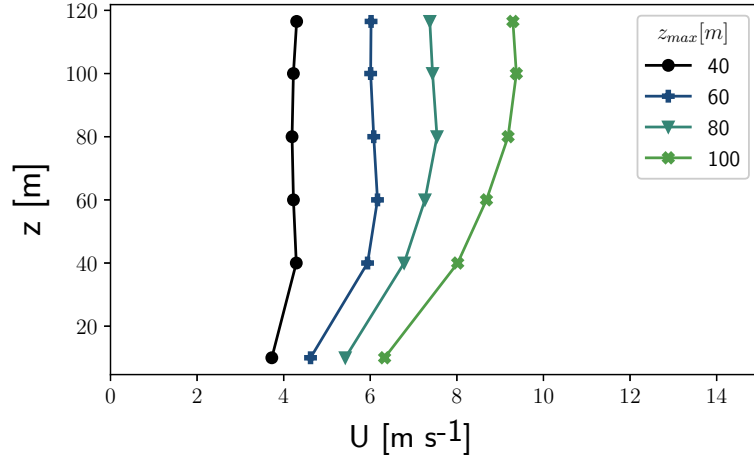
Høvsøre, neutral conditions
