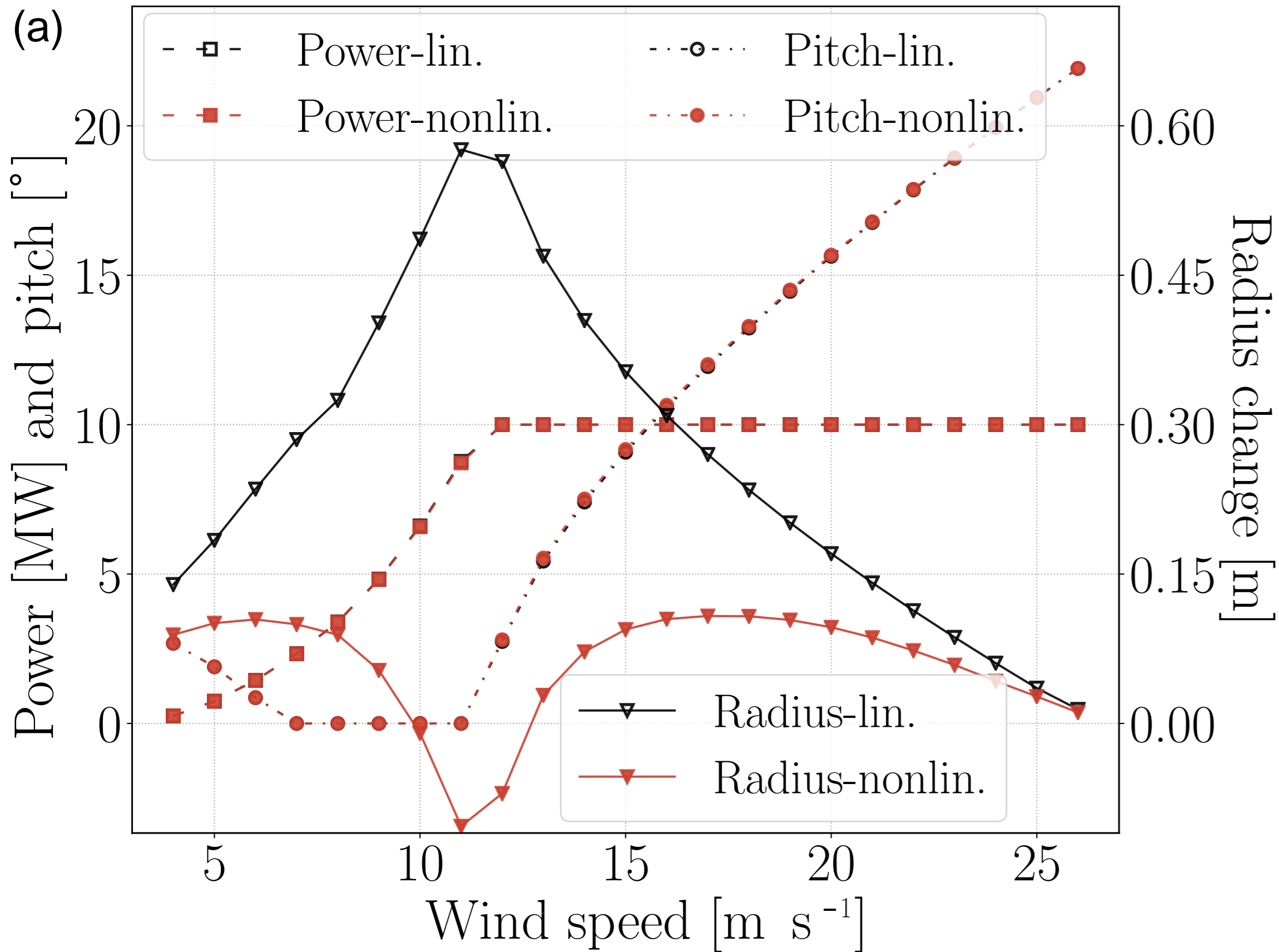
DTU10MW blade
